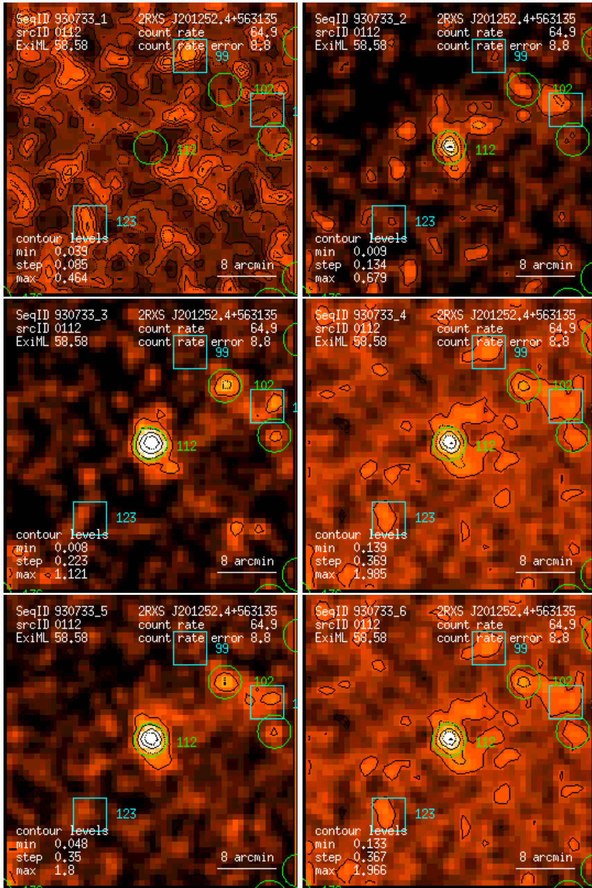
Figure 112: RASS 930733: detection 0112: band rate images, Gaussian filter: (1) PSPC channels 11 – 41, (2) 52 – 90, (3) 91 – 201, (4) 11 – 235, (5) 52 – 201, (6) 11 – 201. Broad band rates in counts/ks. Band rate contour levels in counts/ks/arcmin 2 .
