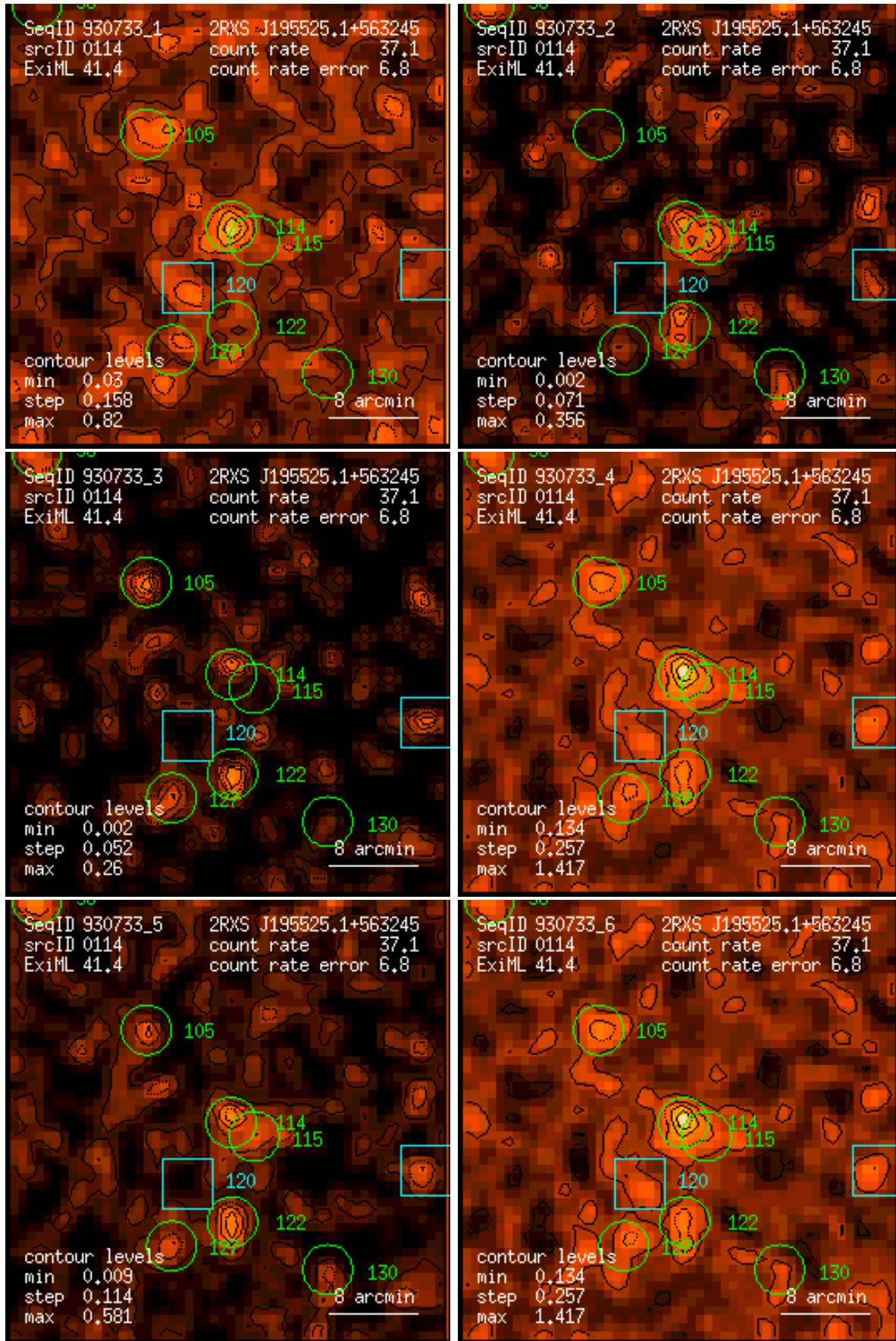
Figure 114: RASS 930733: detection 0114: band rate images, Gaussian filter: (1) PSPC channels 11 – 41, (2) 52 – 90, (3) 91 – 201, (4) 11 – 235, (5) 52 – 201, (6) 11 – 201. Broad band rates in counts/ks. Band rate contour levels in counts/ks/arcmin 2 .
