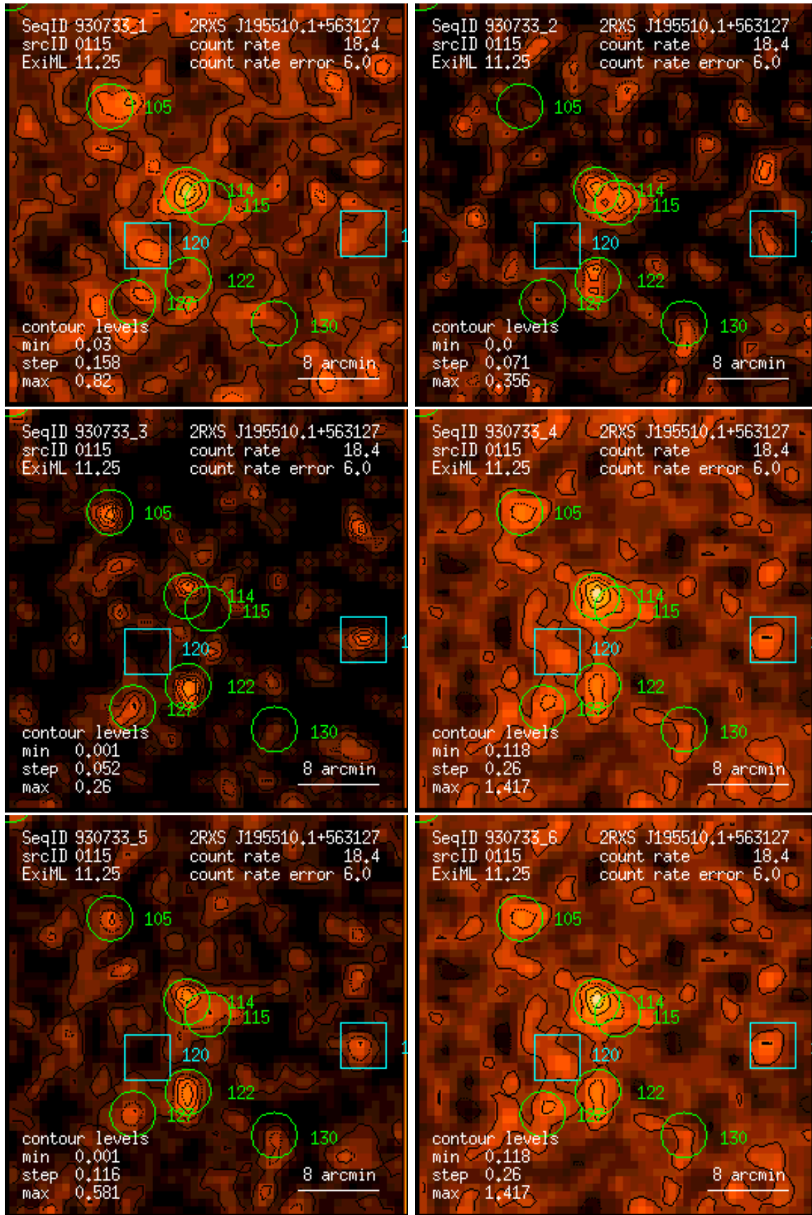
Figure 115: RASS 930733: detection 0115: band rate images, Gaussian filter: (1) PSPC channels 11 – 41, (2) 52 – 90, (3) 91 – 201, (4) 11 – 235, (5) 52 – 201, (6) 11 – 201. Broad band rates in counts/ks. Band rate contour levels in counts/ks/arcmin 2 .
