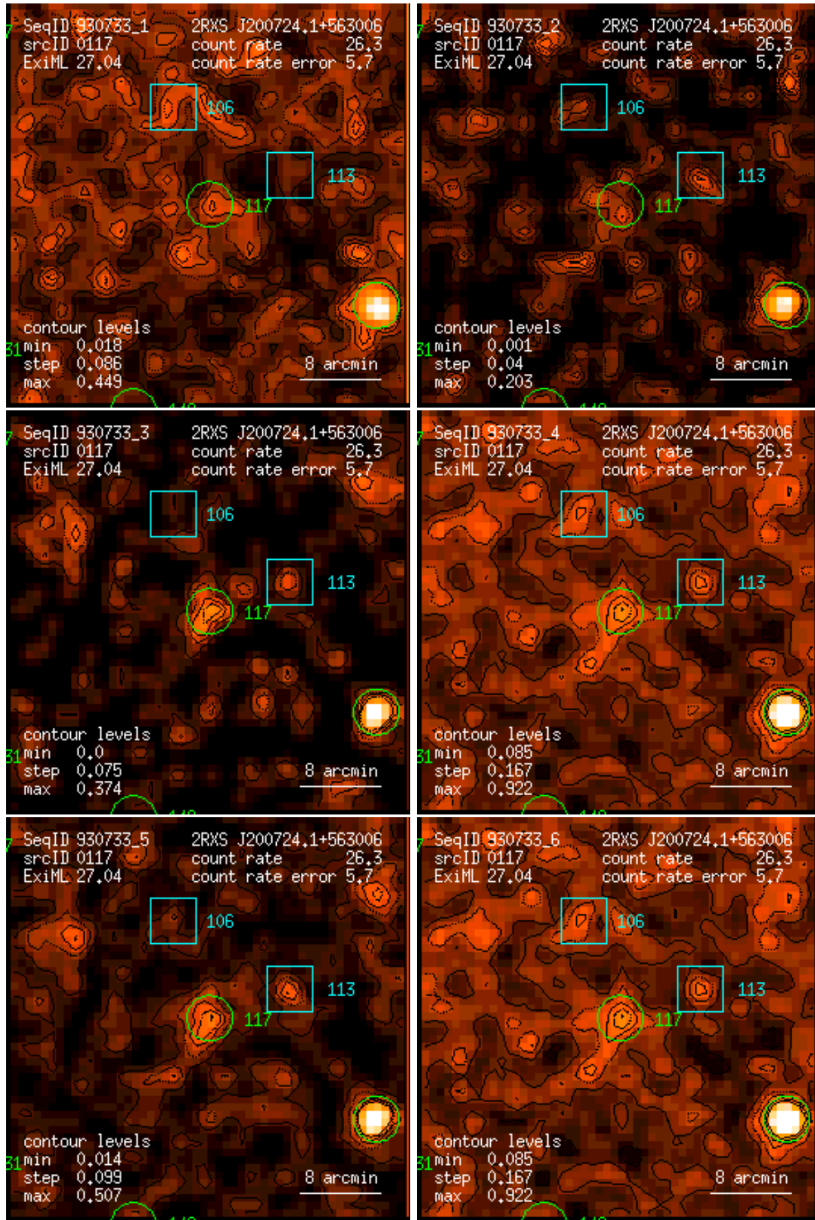
Figure 117: RASS 930733: detection 0117: band rate images, Gaussian filter: (1) PSPC channels 11 – 41, (2) 52 – 90, (3) 91 – 201, (4) 11 – 235, (5) 52 – 201, (6) 11 – 201. Broad band rates in counts/ks. Band rate contour levels in counts/ks/arcmin 2 .
