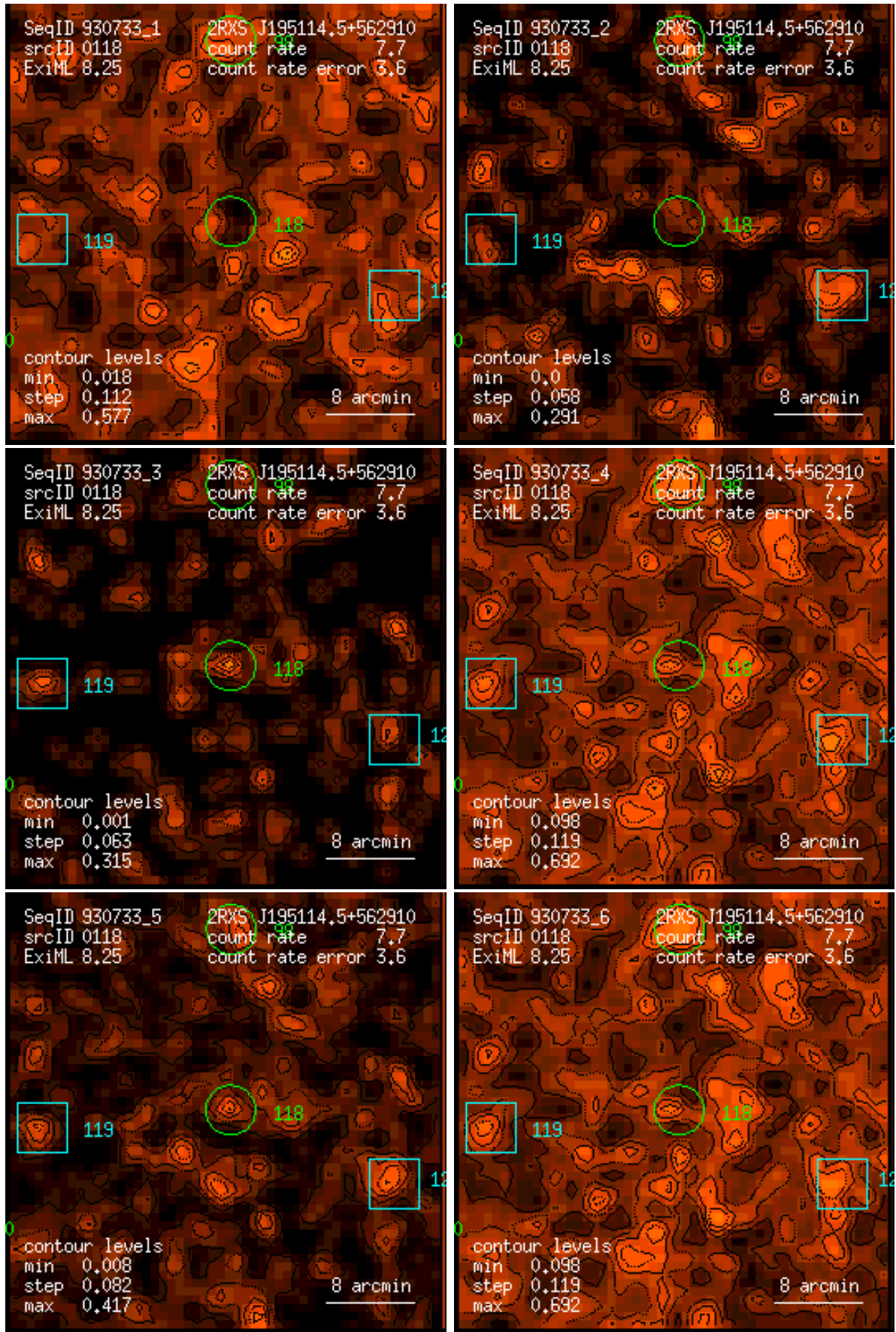
Figure 118: RASS 930733: detection 0118: band rate images, Gaussian filter: (1) PSPC channels 11 – 41, (2) 52 – 90, (3) 91 – 201, (4) 11 – 235, (5) 52 – 201, (6) 11 – 201. Broad band rates in counts/ks. Band rate contour levels in counts/ks/arcmin 2 .
