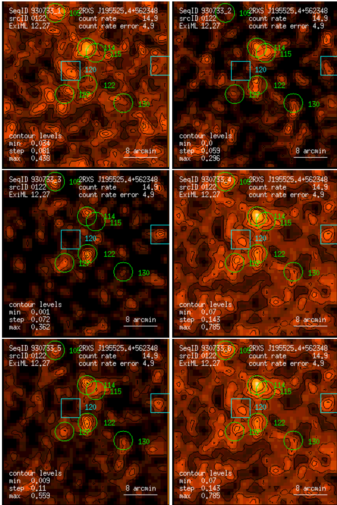
Figure 122: RASS 930733: detection 0122: band rate images, Gaussian filter: (1) PSPC channels 11 – 41, (2) 52 – 90, (3) 91 – 201, (4) 11 – 235, (5) 52 – 201, (6) 11 – 201. Broad band rates in counts/ks. Band rate contour levels in counts/ks/arcmin 2 .
