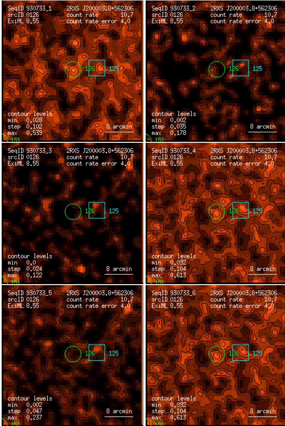
Figure 126: RASS 930733: detection 0126: band rate images, Gaussian filter: (1) PSPC channels 11 – 41, (2) 52 – 90, (3) 91 – 201, (4) 11 – 235, (5) 52 – 201, (6) 11 – 201. Broad band rates in counts/ks. Band rate contour levels in counts/ks/arcmin 2 .
