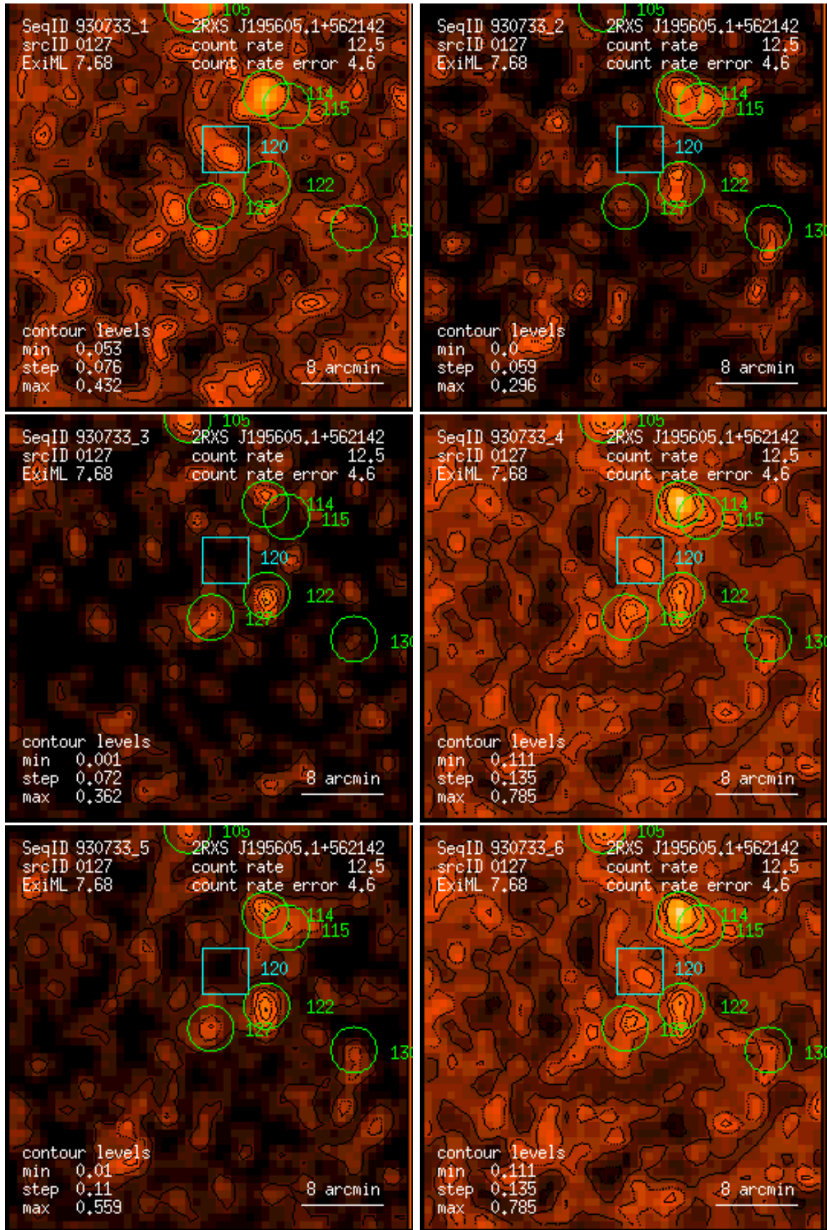
Figure 127: RASS 930733: detection 0127: band rate images, Gaussian filter: (1) PSPC channels 11 – 41, (2) 52 – 90, (3) 91 – 201, (4) 11 – 235, (5) 52 – 201, (6) 11 – 201. Broad band rates in counts/ks. Band rate contour levels in counts/ks/arcmin 2 .
