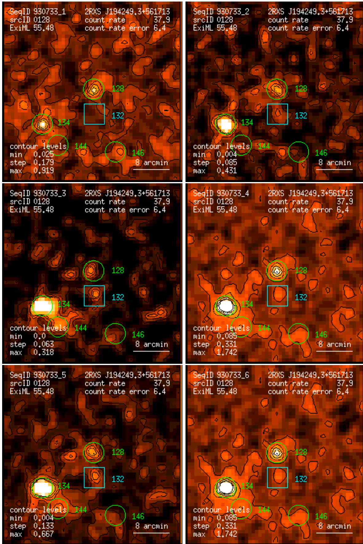
Figure 128: RASS 930733: detection 0128: band rate images, Gaussian filter: (1) PSPC channels 11 – 41, (2) 52 – 90, (3) 91 – 201, (4) 11 – 235, (5) 52 – 201, (6) 11 – 201. Broad band rates in counts/ks. Band rate contour levels in counts/ks/arcmin 2 .
