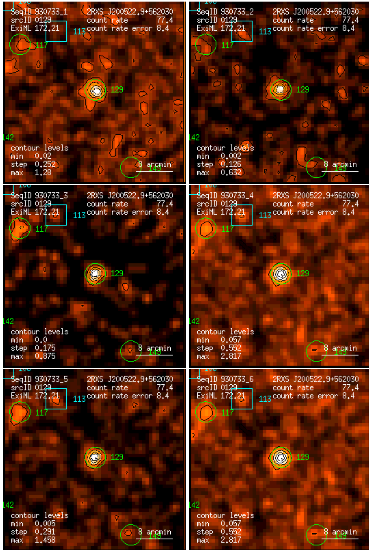
Figure 129: RASS 930733: detection 0129: band rate images, Gaussian filter: (1) PSPC channels 11 – 41, (2) 52 – 90, (3) 91 – 201, (4) 11 – 235, (5) 52 – 201, (6) 11 – 201. Broad band rates in counts/ks. Band rate contour levels in counts/ks/arcmin 2 .
