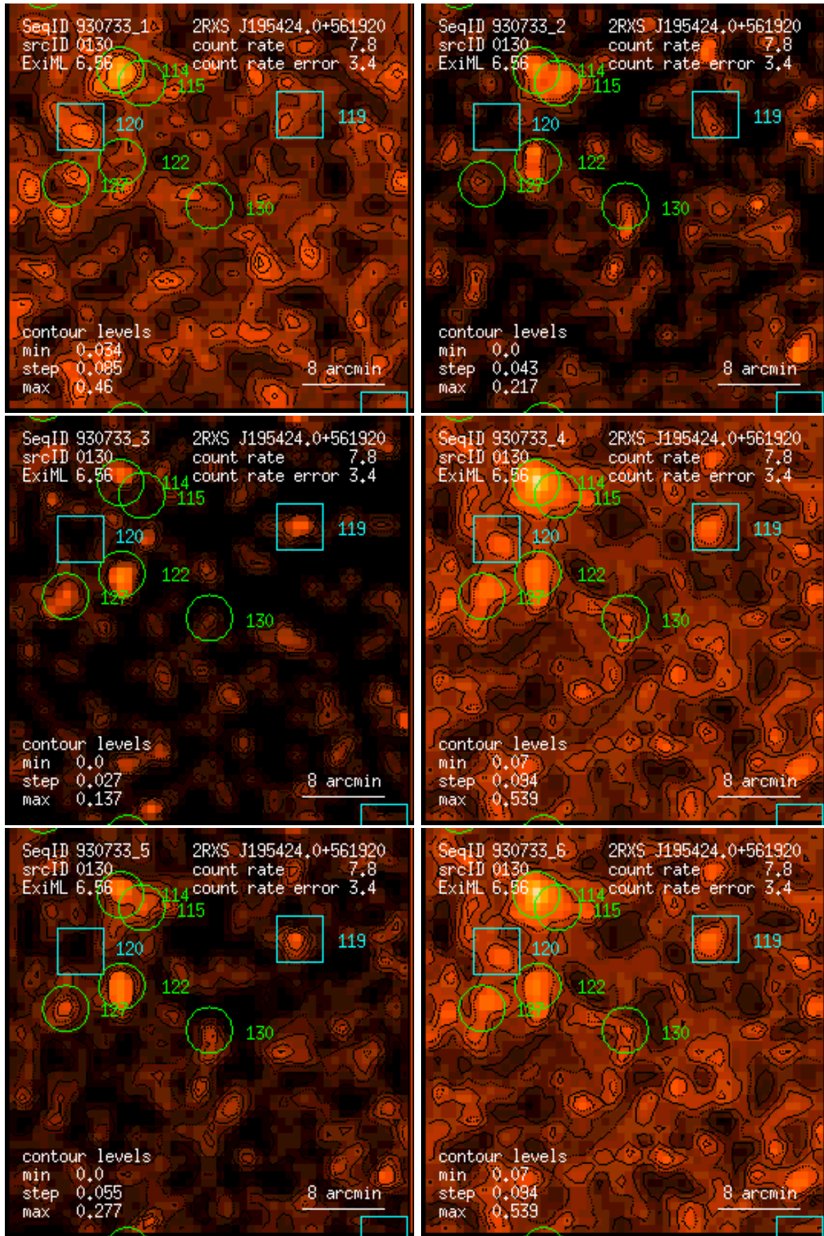
Figure 130: RASS 930733: detection 0130: band rate images, Gaussian filter: (1) PSPC channels 11 – 41, (2) 52 – 90, (3) 91 – 201, (4) 11 – 235, (5) 52 – 201, (6) 11 – 201. Broad band rates in counts/ks. Band rate contour levels in counts/ks/arcmin 2 .
