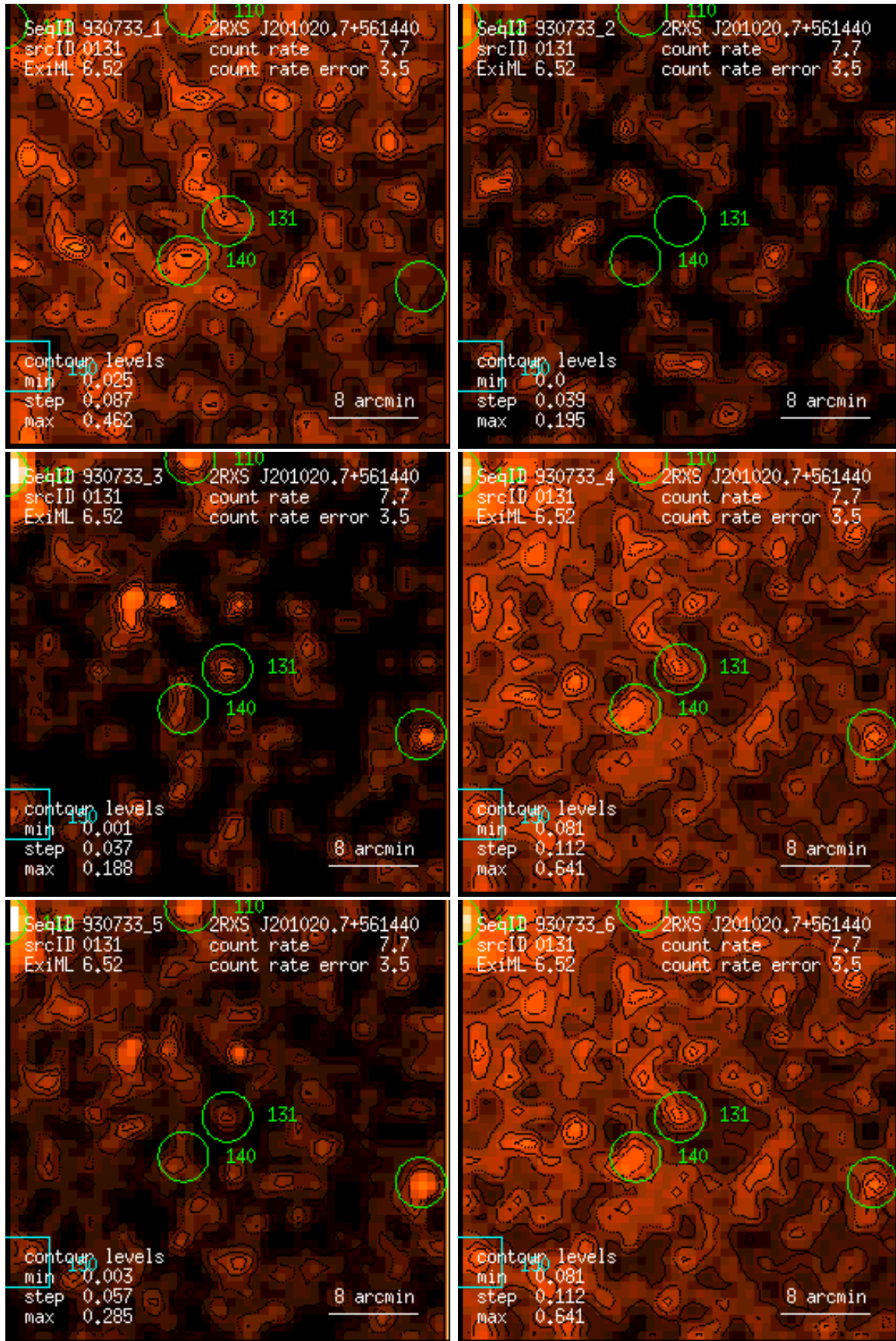
Figure 131: RASS 930733: detection 0131: band rate images, Gaussian filter: (1) PSPC channels 11 – 41, (2) 52 – 90, (3) 91 – 201, (4) 11 – 235, (5) 52 – 201, (6) 11 – 201. Broad band rates in counts/ks. Band rate contour levels in counts/ks/arcmin 2 .
