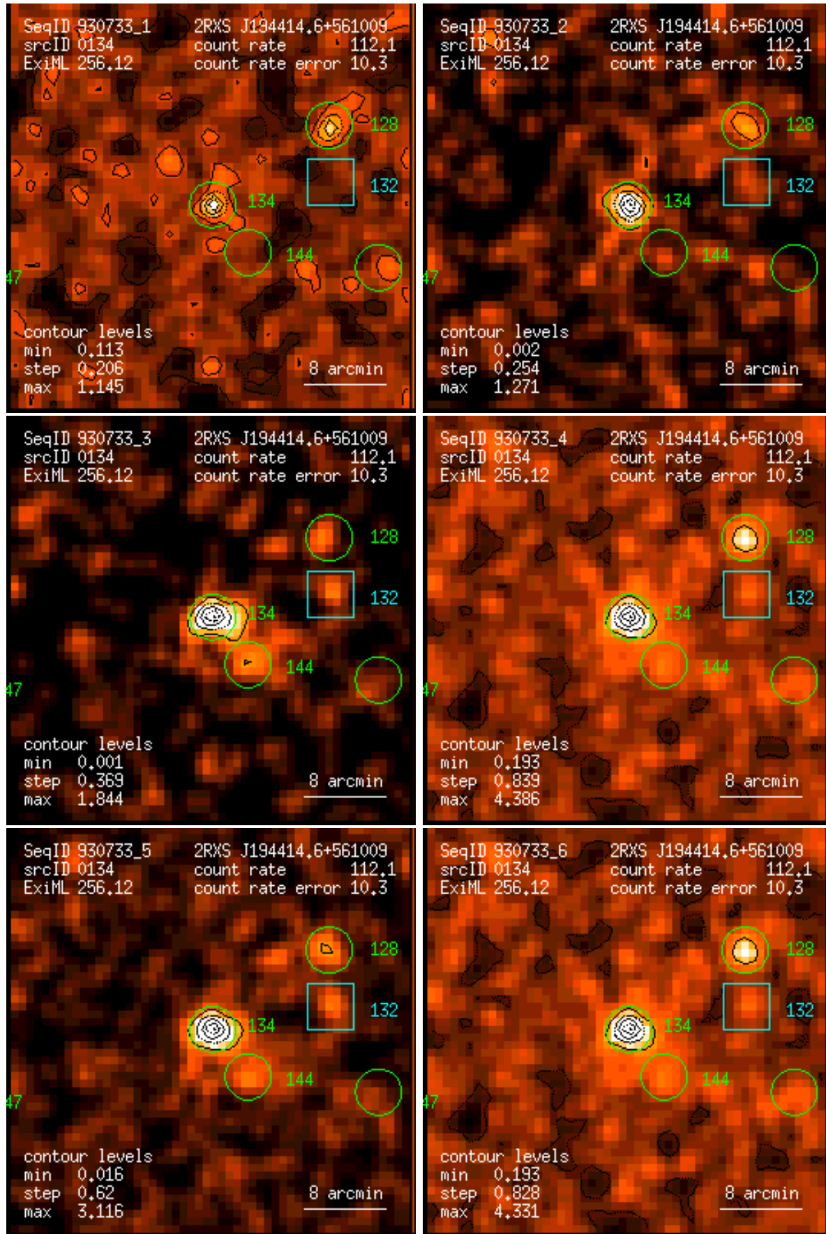
Figure 134: RASS 930733: detection 0134: band rate images, Gaussian filter: (1) PSPC channels 11 – 41, (2) 52 – 90, (3) 91 – 201, (4) 11 – 235, (5) 52 – 201, (6) 11 – 201. Broad band rates in counts/ks. Band rate contour levels in counts/ks/arcmin 2 .
