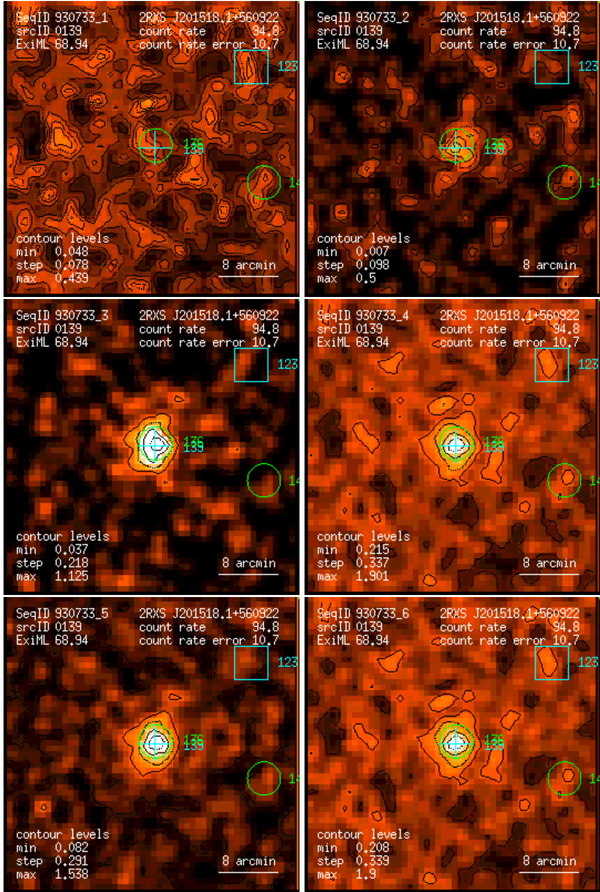
Figure 139: RASS 930733: detection 0139: band rate images, Gaussian filter: (1) PSPC channels 11 – 41, (2) 52 – 90, (3) 91 – 201, (4) 11 – 235, (5) 52 – 201, (6) 11 – 201. Broad band rates in counts/ks. Band rate contour levels in counts/ks/arcmin 2 .
