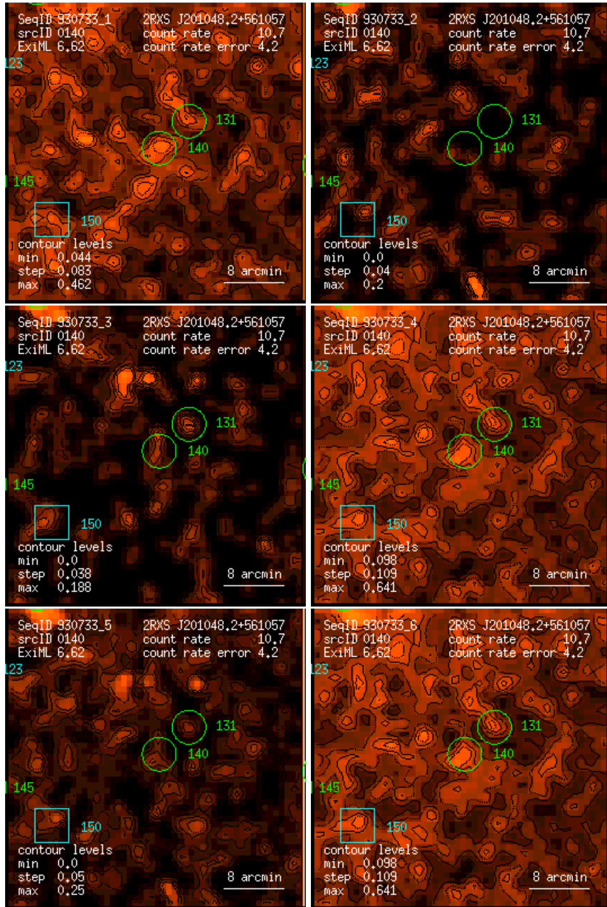
Figure 140: RASS 930733: detection 0140: band rate images, Gaussian filter: (1) PSPC channels 11 – 41, (2) 52 – 90, (3) 91 – 201, (4) 11 – 235, (5) 52 – 201, (6) 11 – 201. Broad band rates in counts/ks. Band rate contour levels in counts/ks/arcmin 2 .
