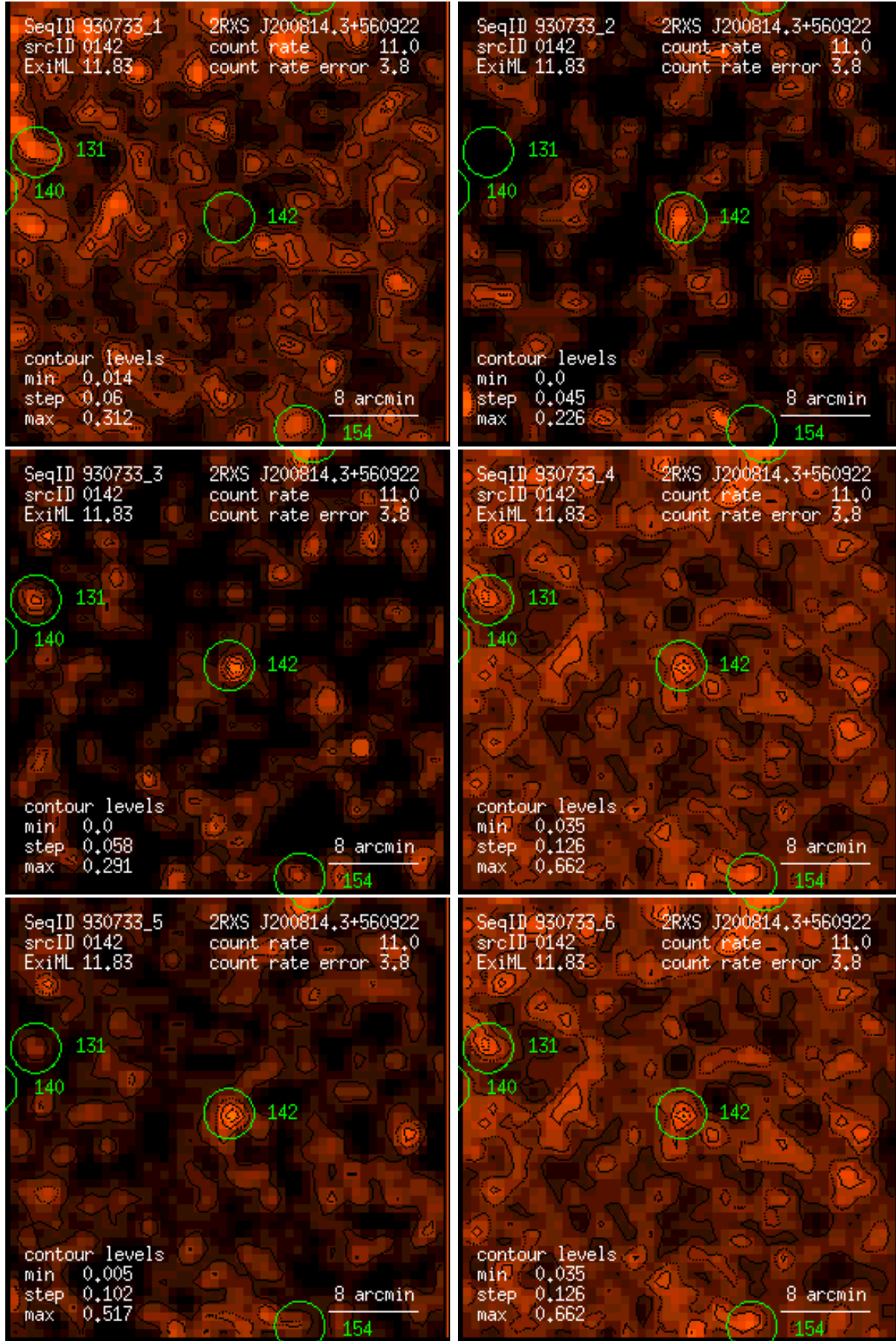
Figure 142: RASS 930733: detection 0142: band rate images, Gaussian filter: (1) PSPC channels 11 – 41, (2) 52 – 90, (3) 91 – 201, (4) 11 – 235, (5) 52 – 201, (6) 11 – 201. Broad band rates in counts/ks. Band rate contour levels in counts/ks/arcmin 2 .
