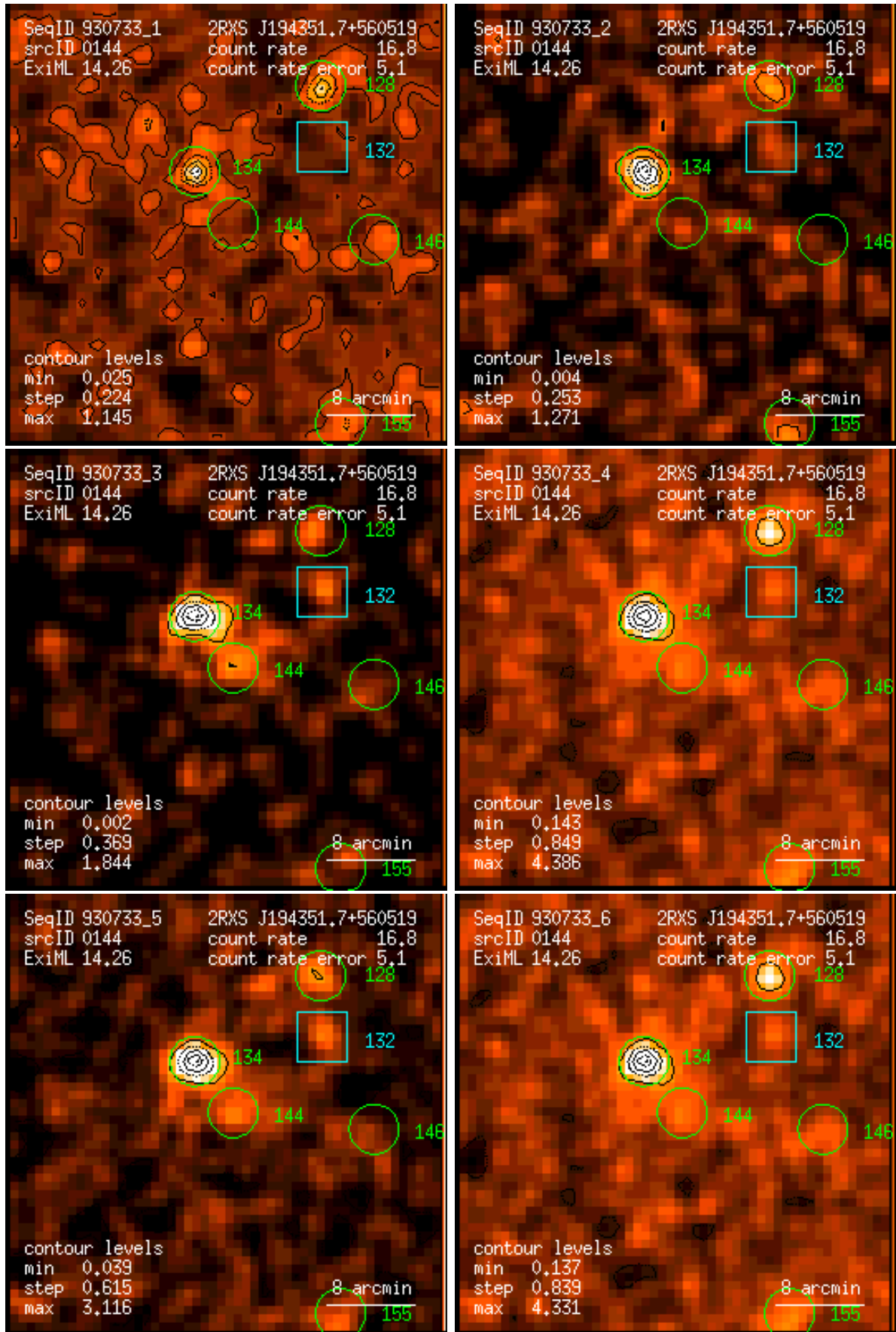
Figure 144: RASS 930733: detection 0144: band rate images, Gaussian filter: (1) PSPC channels 11 – 41, (2) 52 – 90, (3) 91 – 201, (4) 11 – 235, (5) 52 – 201, (6) 11 – 201. Broad band rates in counts/ks. Band rate contour levels in counts/ks/arcmin 2 .
