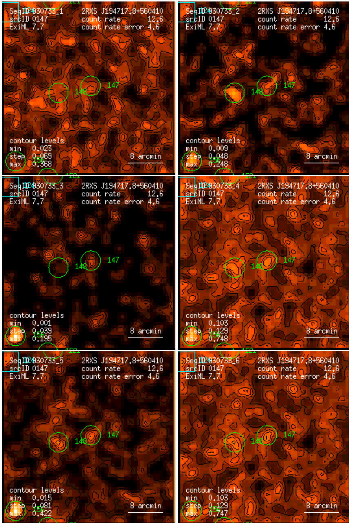
Figure 147: RASS 930733: detection 0147: band rate images, Gaussian filter: (1) PSPC channels 11 – 41, (2) 52 – 90, (3) 91 – 201, (4) 11 – 235, (5) 52 – 201, (6) 11 – 201. Broad band rates in counts/ks. Band rate contour levels in counts/ks/arcmin 2 .
