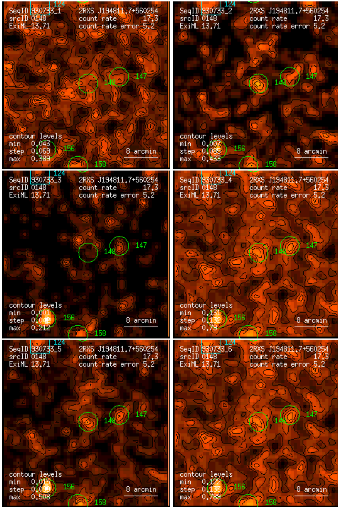
Figure 148: RASS 930733: detection 0148: band rate images, Gaussian filter: (1) PSPC channels 11 – 41, (2) 52 – 90, (3) 91 – 201, (4) 11 – 235, (5) 52 – 201, (6) 11 – 201. Broad band rates in counts/ks. Band rate contour levels in counts/ks/arcmin 2 .
