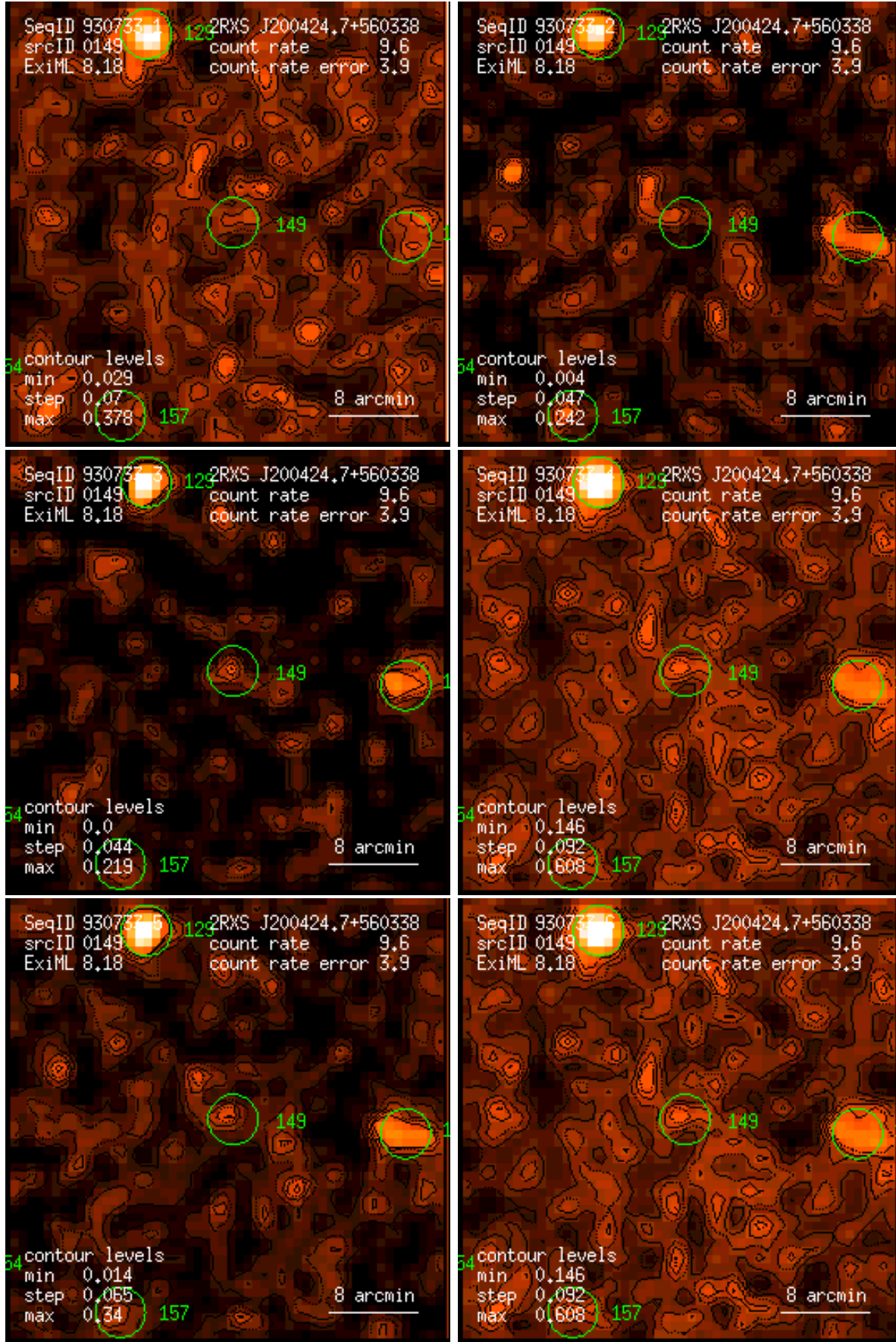
Figure 149: RASS 930733: detection 0149: band rate images, Gaussian filter: (1) PSPC channels 11 – 41, (2) 52 – 90, (3) 91 – 201, (4) 11 – 235, (5) 52 – 201, (6) 11 – 201. Broad band rates in counts/ks. Band rate contour levels in counts/ks/arcmin 2 .
