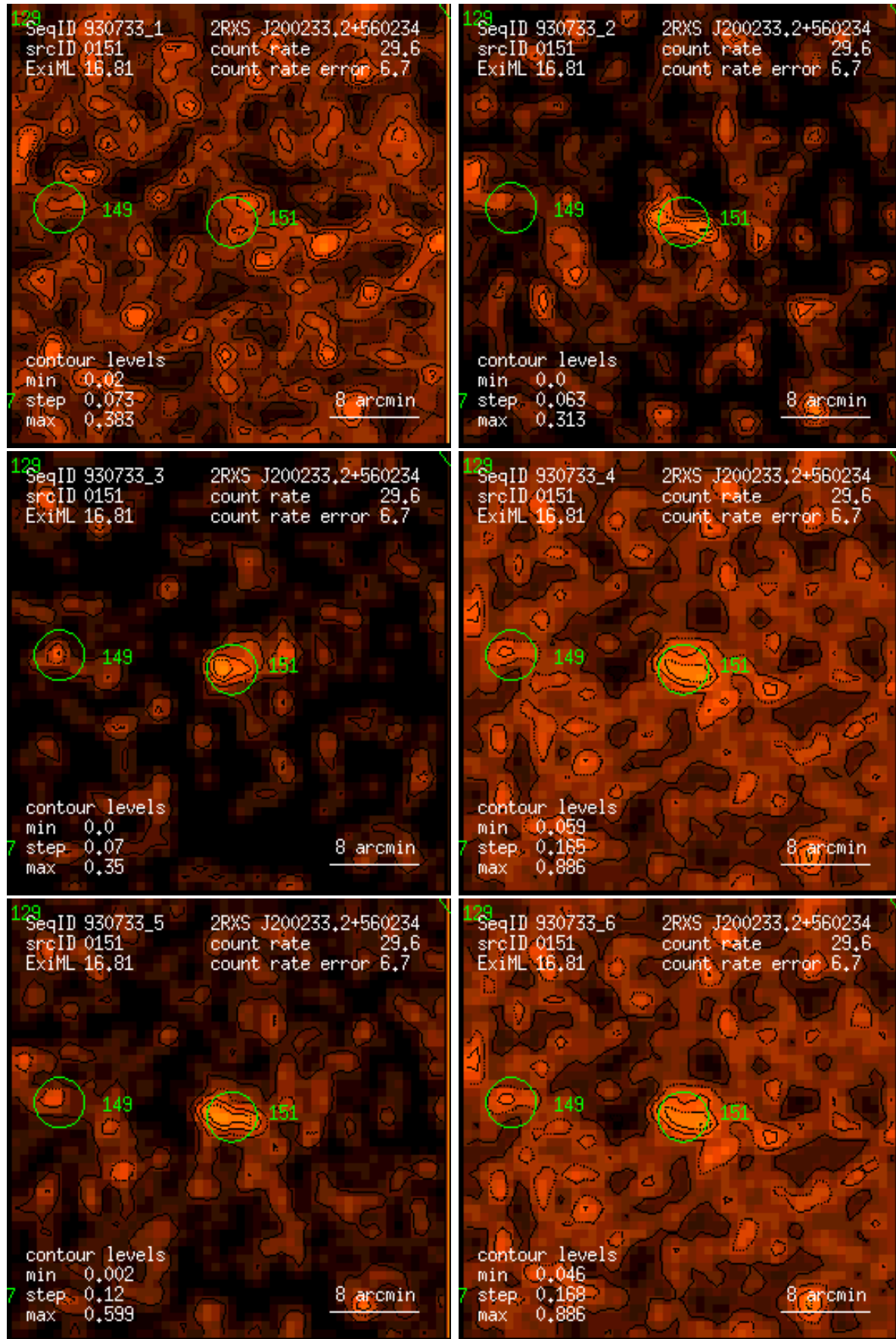
Figure 151: RASS 930733: detection 0151: band rate images, Gaussian filter: (1) PSPC channels 11 – 41, (2) 52 – 90, (3) 91 – 201, (4) 11 – 235, (5) 52 – 201, (6) 11 – 201. Broad band rates in counts/ks. Band rate contour levels in counts/ks/arcmin 2 .
