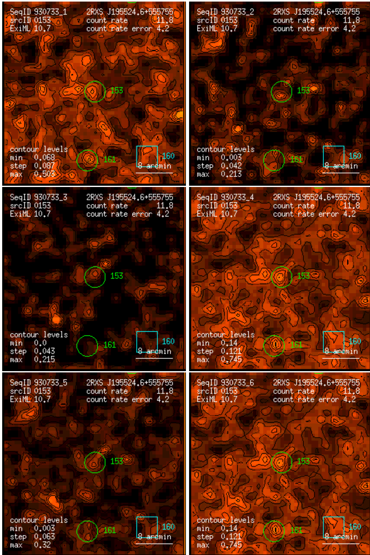
Figure 153: RASS 930733: detection 0153: band rate images, Gaussian filter: (1) PSPC channels 11 – 41, (2) 52 – 90, (3) 91 – 201, (4) 11 – 235, (5) 52 – 201, (6) 11 – 201. Broad band rates in counts/ks. Band rate contour levels in counts/ks/arcmin 2 .
