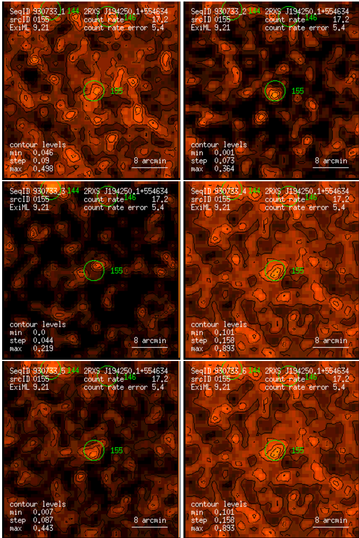
Figure 155: RASS 930733: detection 0155: band rate images, Gaussian filter: (1) PSPC channels 11 – 41, (2) 52 – 90, (3) 91 – 201, (4) 11 – 235, (5) 52 – 201, (6) 11 – 201. Broad band rates in counts/ks. Band rate contour levels in counts/ks/arcmin 2 .
