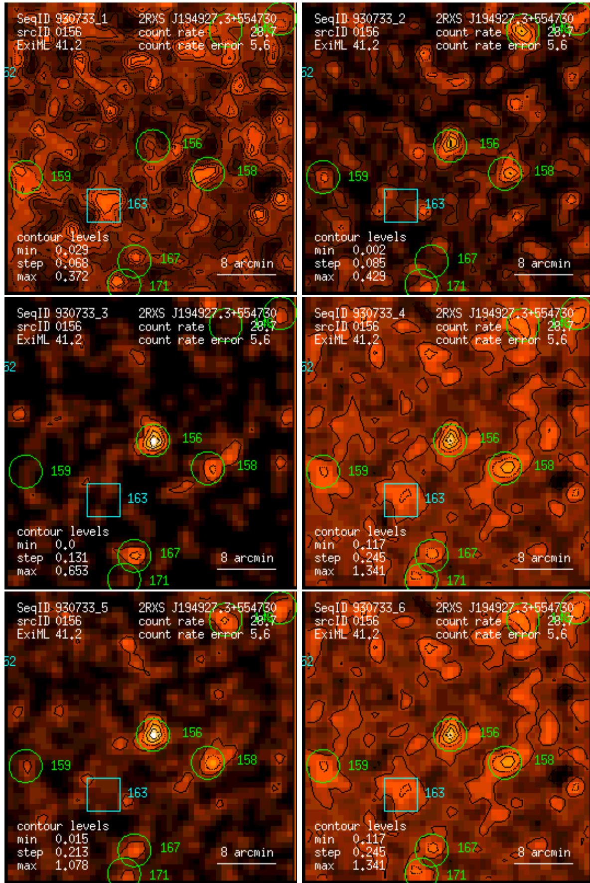
Figure 156: RASS 930733: detection 0156: band rate images, Gaussian filter: (1) PSPC channels 11 – 41, (2) 52 – 90, (3) 91 – 201, (4) 11 – 235, (5) 52 – 201, (6) 11 – 201. Broad band rates in counts/ks. Band rate contour levels in counts/ks/arcmin 2 .
