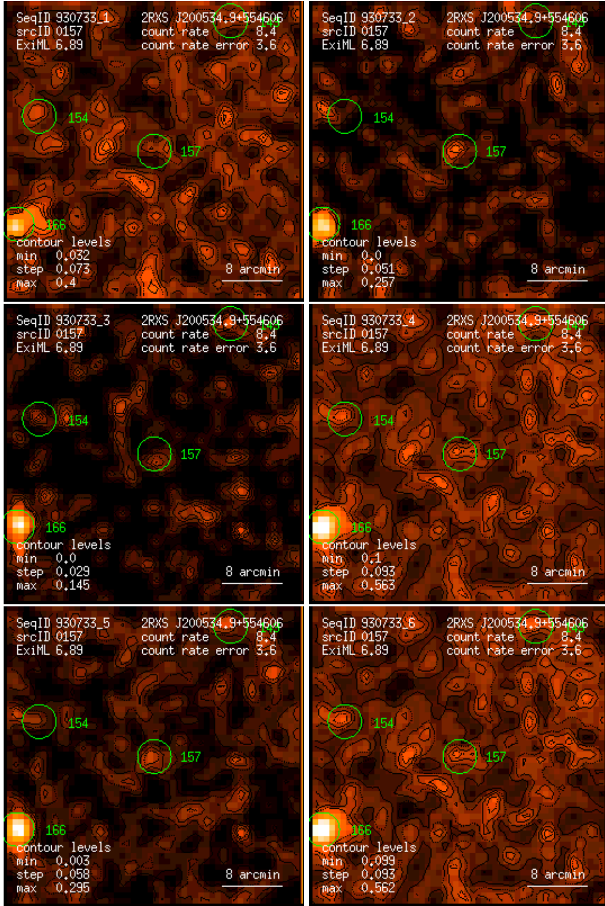
Figure 157: RASS 930733: detection 0157: band rate images, Gaussian filter: (1) PSPC channels 11 – 41, (2) 52 – 90, (3) 91 – 201, (4) 11 – 235, (5) 52 – 201, (6) 11 – 201. Broad band rates in counts/ks. Band rate contour levels in counts/ks/arcmin 2 .
