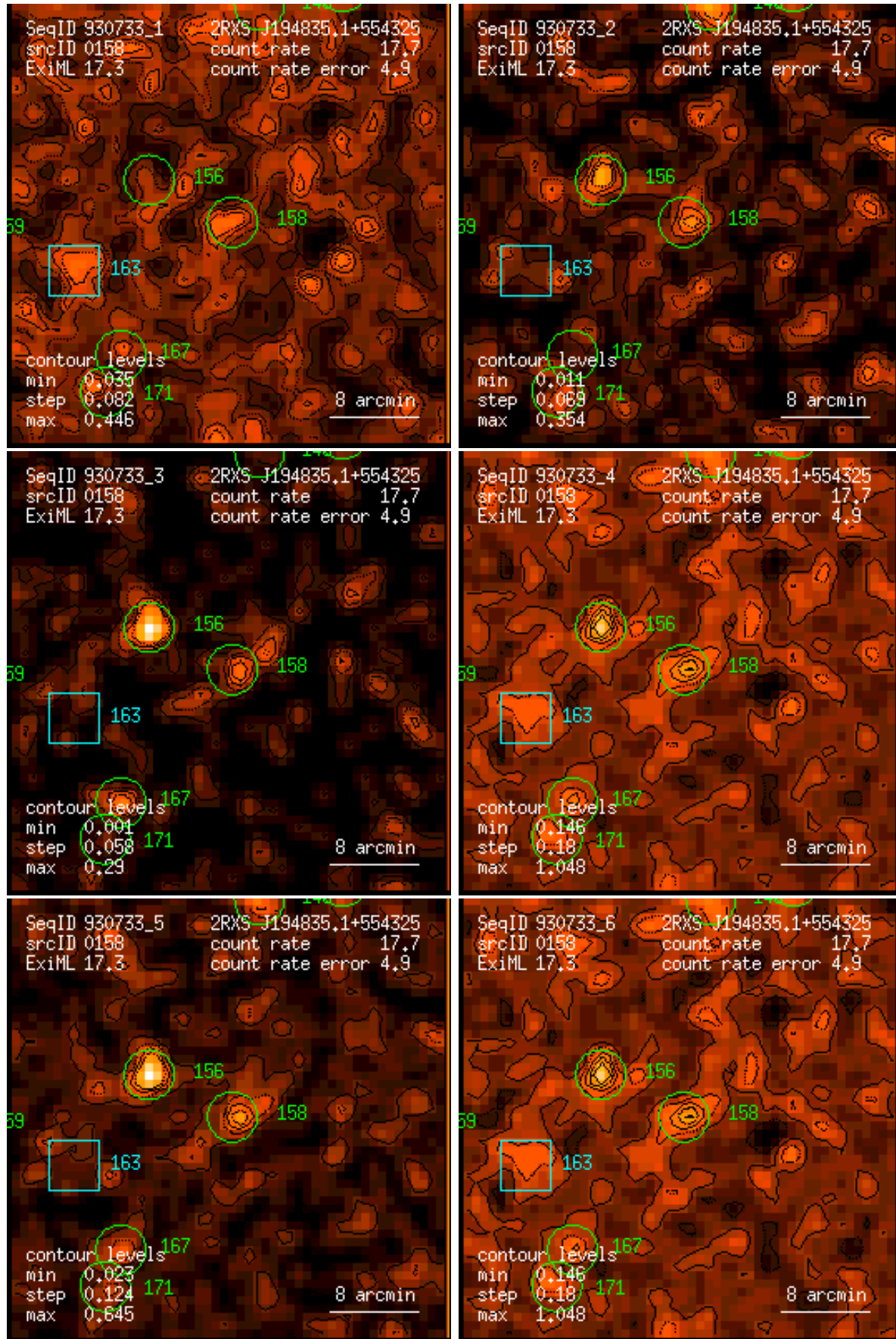
Figure 158: RASS 930733: detection 0158: band rate images, Gaussian filter: (1) PSPC channels 11 – 41, (2) 52 – 90, (3) 91 – 201, (4) 11 – 235, (5) 52 – 201, (6) 11 – 201. Broad band rates in counts/ks. Band rate contour levels in counts/ks/arcmin 2 .
