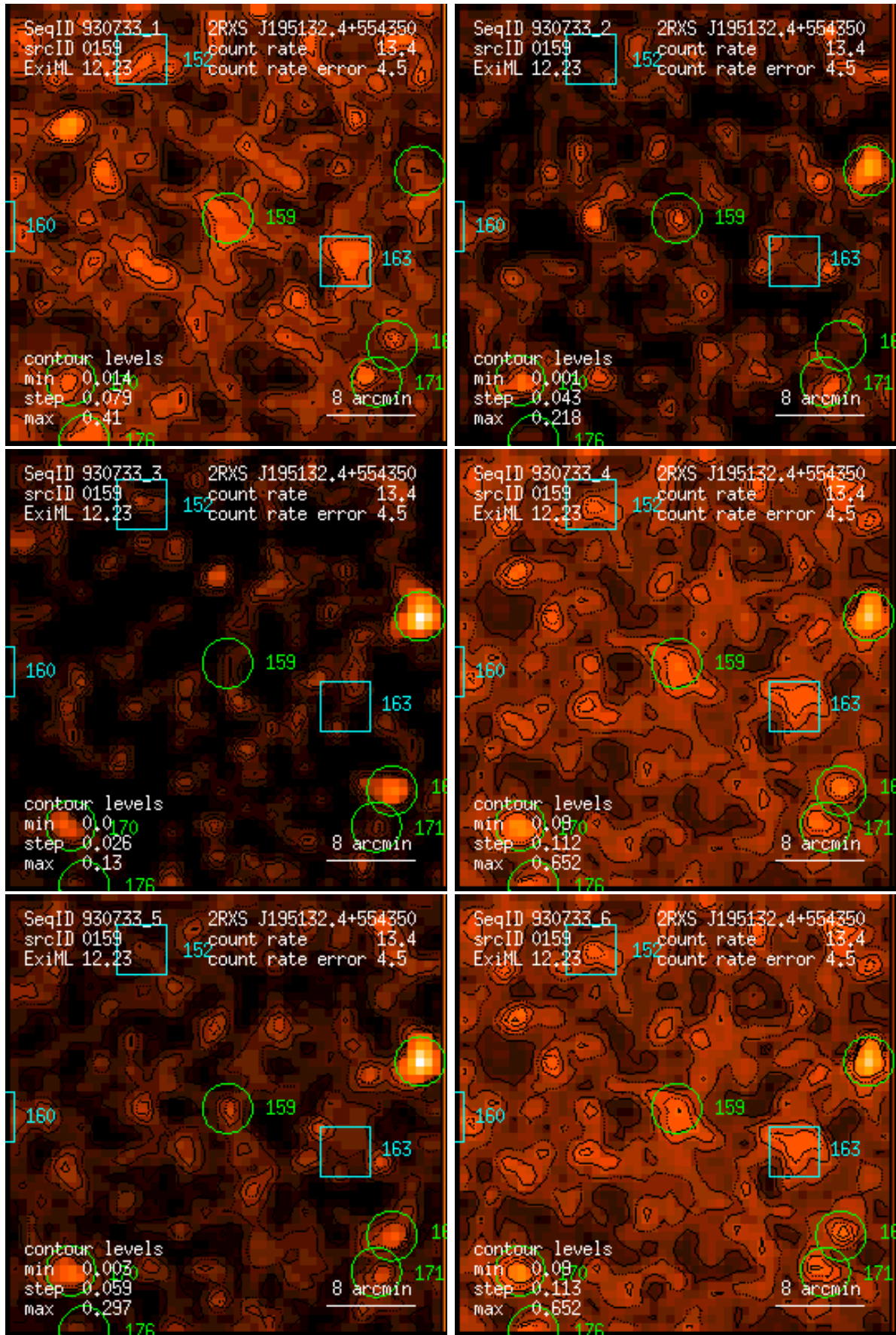
Figure 159: RASS 930733: detection 0159: band rate images, Gaussian filter: (1) PSPC channels 11 – 41, (2) 52 – 90, (3) 91 – 201, (4) 11 – 235, (5) 52 – 201, (6) 11 – 201. Broad band rates in counts/ks. Band rate contour levels in counts/ks/arcmin 2 .
