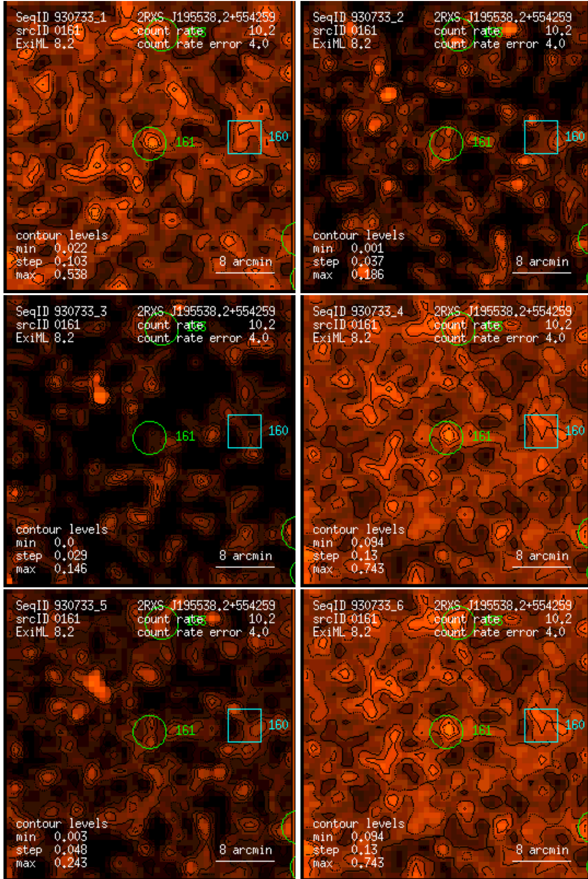
Figure 161: RASS 930733: detection 0161: band rate images, Gaussian filter: (1) PSPC channels 11 – 41, (2) 52 – 90, (3) 91 – 201, (4) 11 – 235, (5) 52 – 201, (6) 11 – 201. Broad band rates in counts/ks. Band rate contour levels in counts/ks/arcmin 2 .
