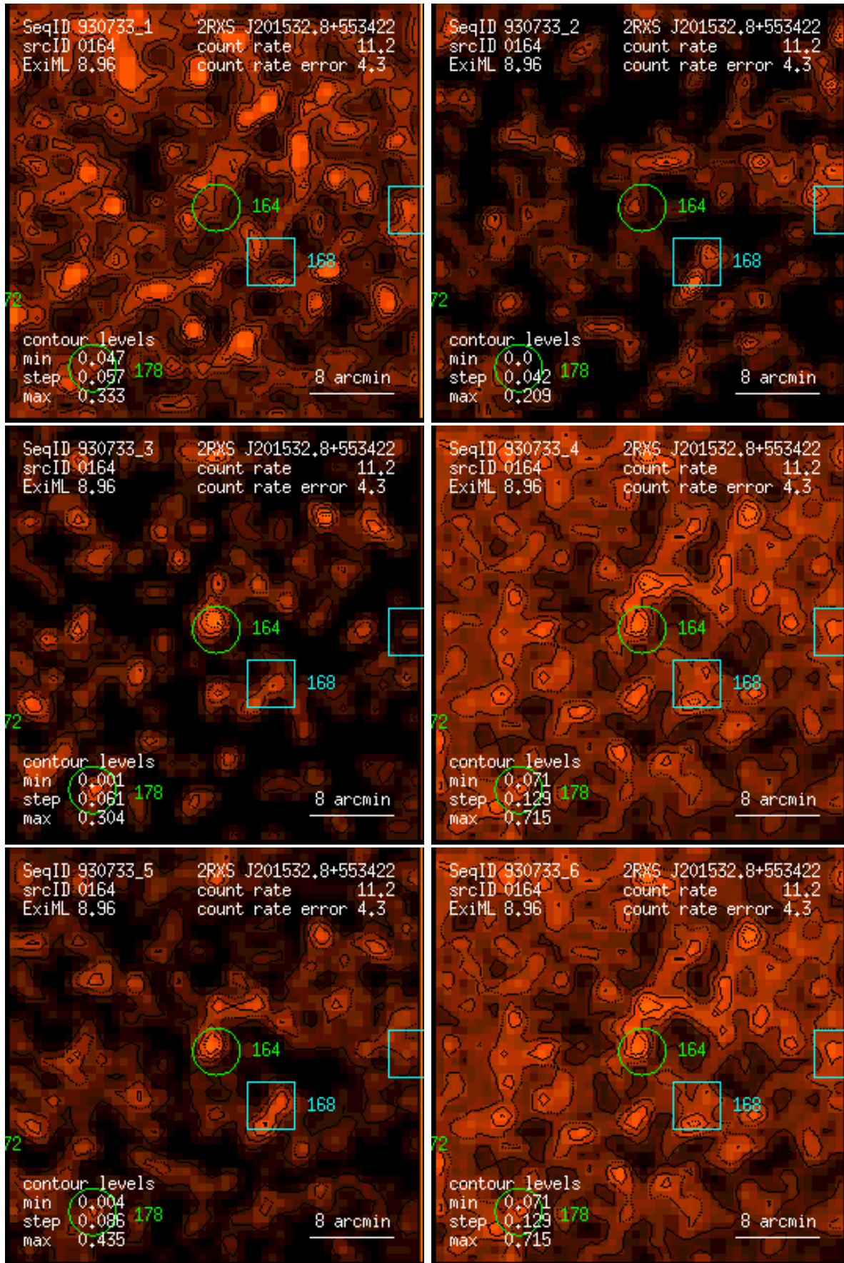
Figure 164: RASS 930733: detection 0164: band rate images, Gaussian filter: (1) PSPC channels 11 – 41, (2) 52 – 90, (3) 91 – 201, (4) 11 – 235, (5) 52 – 201, (6) 11 – 201. Broad band rates in counts/ks. Band rate contour levels in counts/ks/arcmin 2 .
