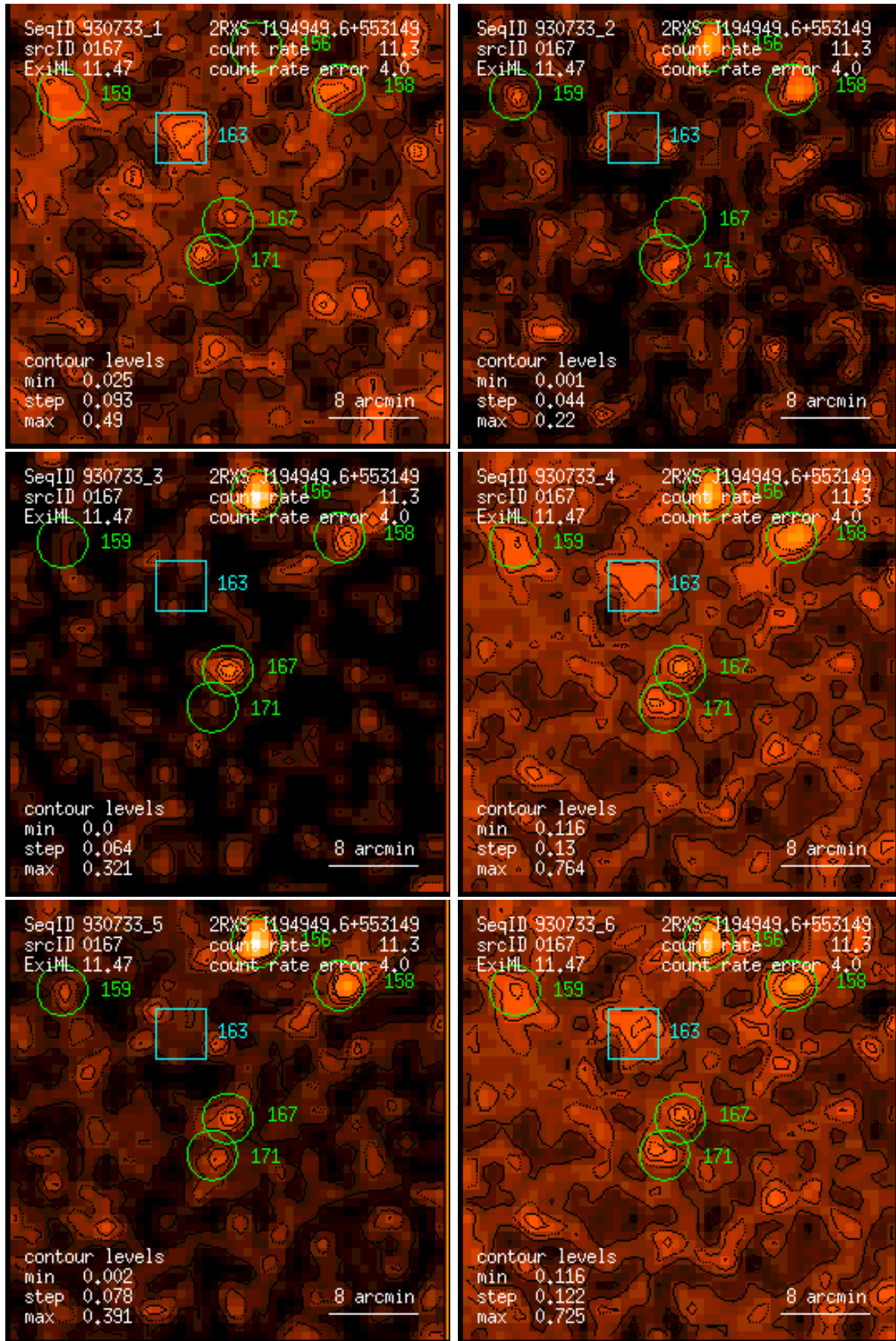
Figure 167: RASS 930733: detection 0167: band rate images, Gaussian filter: (1) PSPC channels 11 – 41, (2) 52 – 90, (3) 91 – 201, (4) 11 – 235, (5) 52 – 201, (6) 11 – 201. Broad band rates in counts/ks. Band rate contour levels in counts/ks/arcmin 2 .
