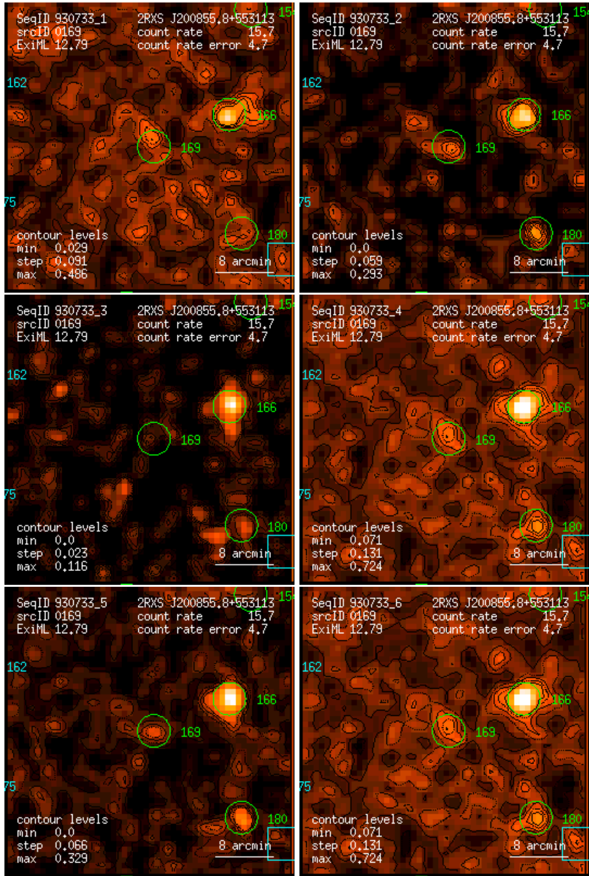
Figure 169: RASS 930733: detection 0169: band rate images, Gaussian filter: (1) PSPC channels 11 – 41, (2) 52 – 90, (3) 91 – 201, (4) 11 – 235, (5) 52 – 201, (6) 11 – 201. Broad band rates in counts/ks. Band rate contour levels in counts/ks/arcmin 2 .
