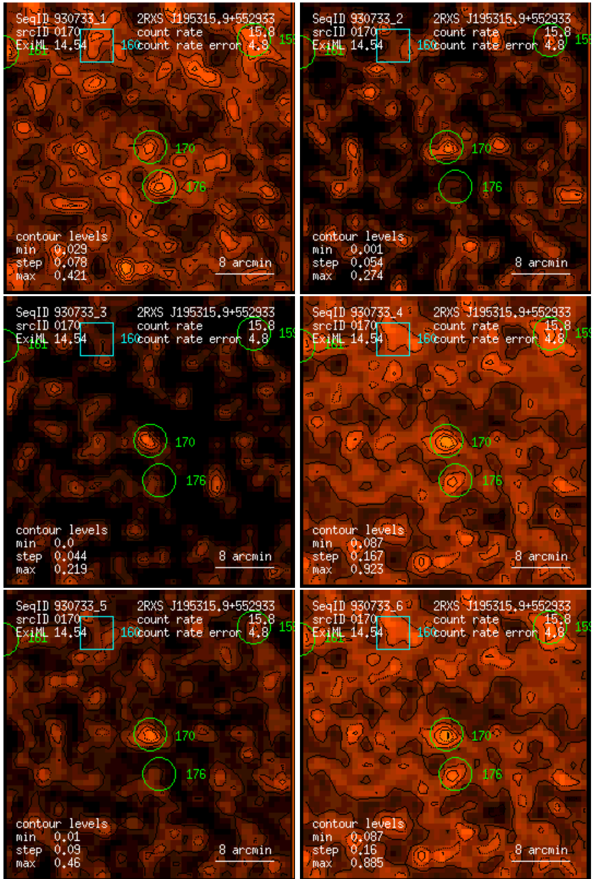
Figure 170: RASS 930733: detection 0170: band rate images, Gaussian filter: (1) PSPC channels 11 – 41, (2) 52 – 90, (3) 91 – 201, (4) 11 – 235, (5) 52 – 201, (6) 11 – 201. Broad band rates in counts/ks. Band rate contour levels in counts/ks/arcmin 2 .
