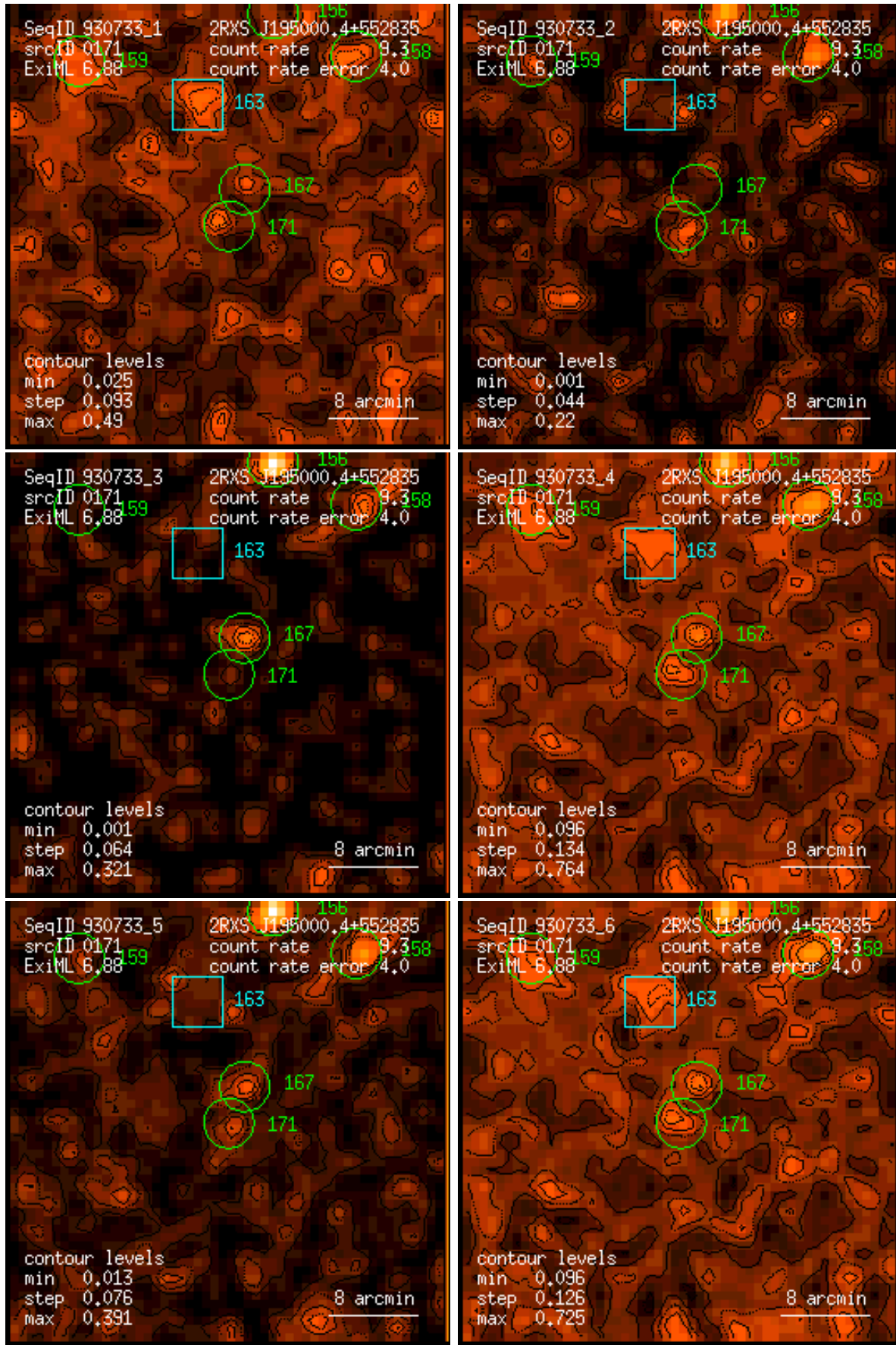
Figure 171: RASS 930733: detection 0171: band rate images, Gaussian filter: (1) PSPC channels 11 – 41, (2) 52 – 90, (3) 91 – 201, (4) 11 – 235, (5) 52 – 201, (6) 11 – 201. Broad band rates in counts/ks. Band rate contour levels in counts/ks/arcmin 2 .
