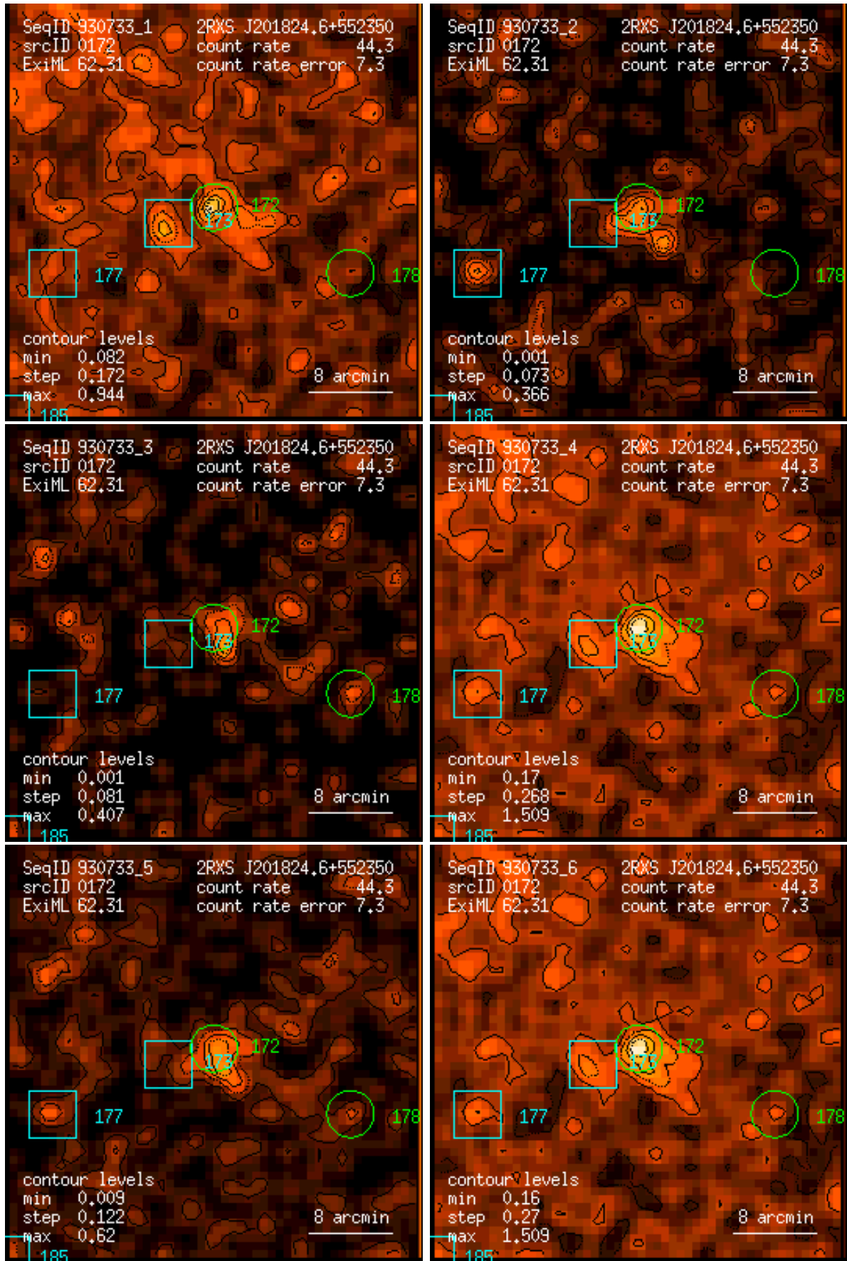
Figure 172: RASS 930733: detection 0172: band rate images, Gaussian filter: (1) PSPC channels 11 – 41, (2) 52 – 90, (3) 91 – 201, (4) 11 – 235, (5) 52 – 201, (6) 11 – 201. Broad band rates in counts/ks. Band rate contour levels in counts/ks/arcmin 2 .
