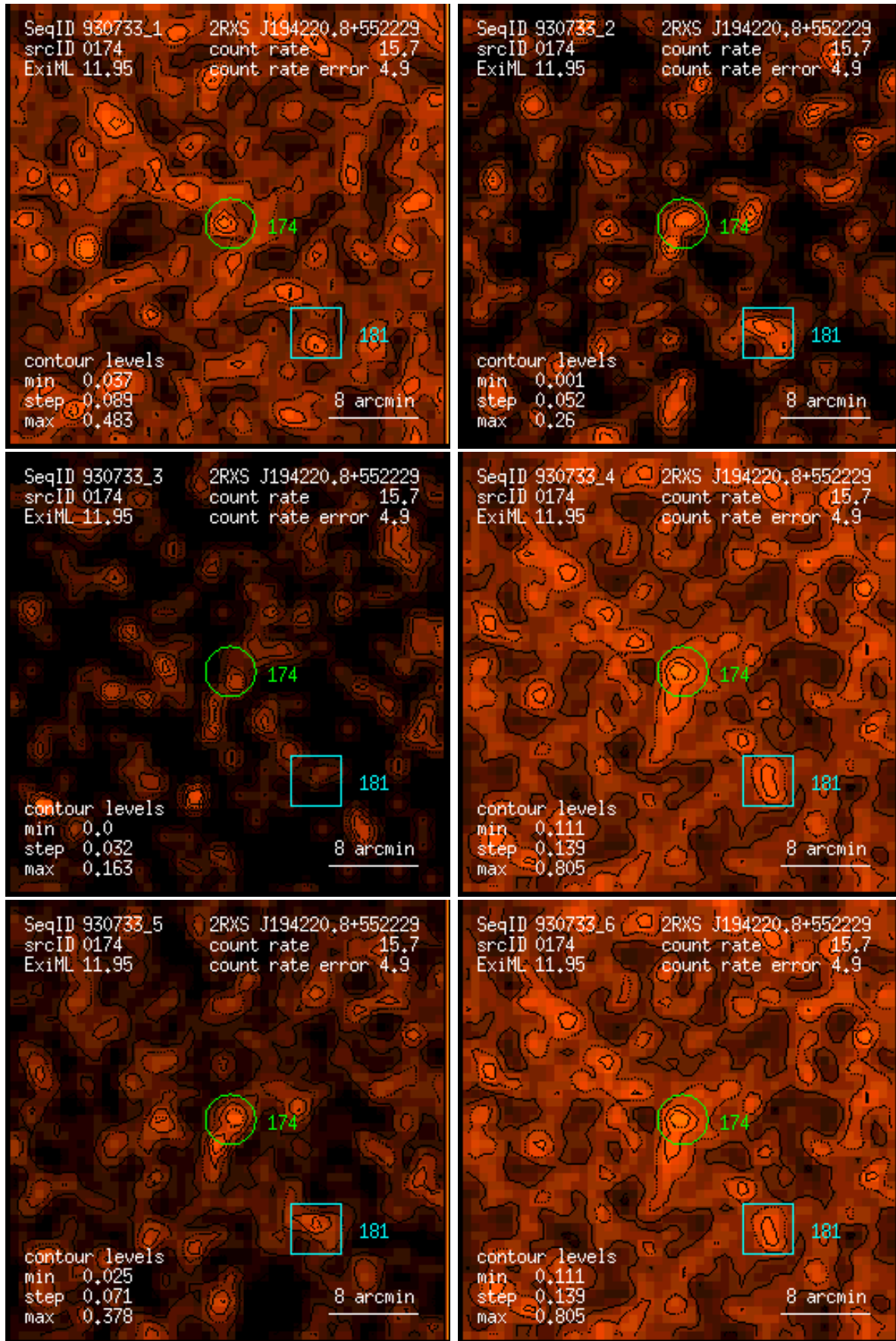
Figure 174: RASS 930733: detection 0174: band rate images, Gaussian filter: (1) PSPC channels 11 – 41, (2) 52 – 90, (3) 91 – 201, (4) 11 – 235, (5) 52 – 201, (6) 11 – 201. Broad band rates in counts/ks. Band rate contour levels in counts/ks/arcmin 2 .
