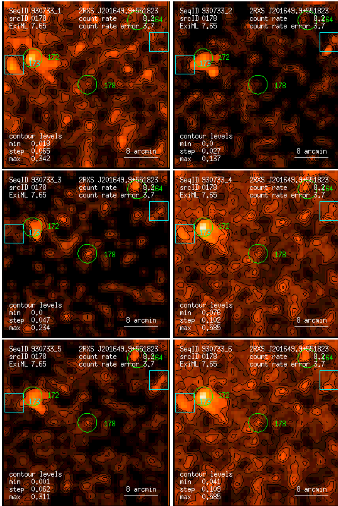
Figure 178: RASS 930733: detection 0178: band rate images, Gaussian filter: (1) PSPC channels 11 – 41, (2) 52 – 90, (3) 91 – 201, (4) 11 – 235, (5) 52 – 201, (6) 11 – 201. Broad band rates in counts/ks. Band rate contour levels in counts/ks/arcmin 2 .
