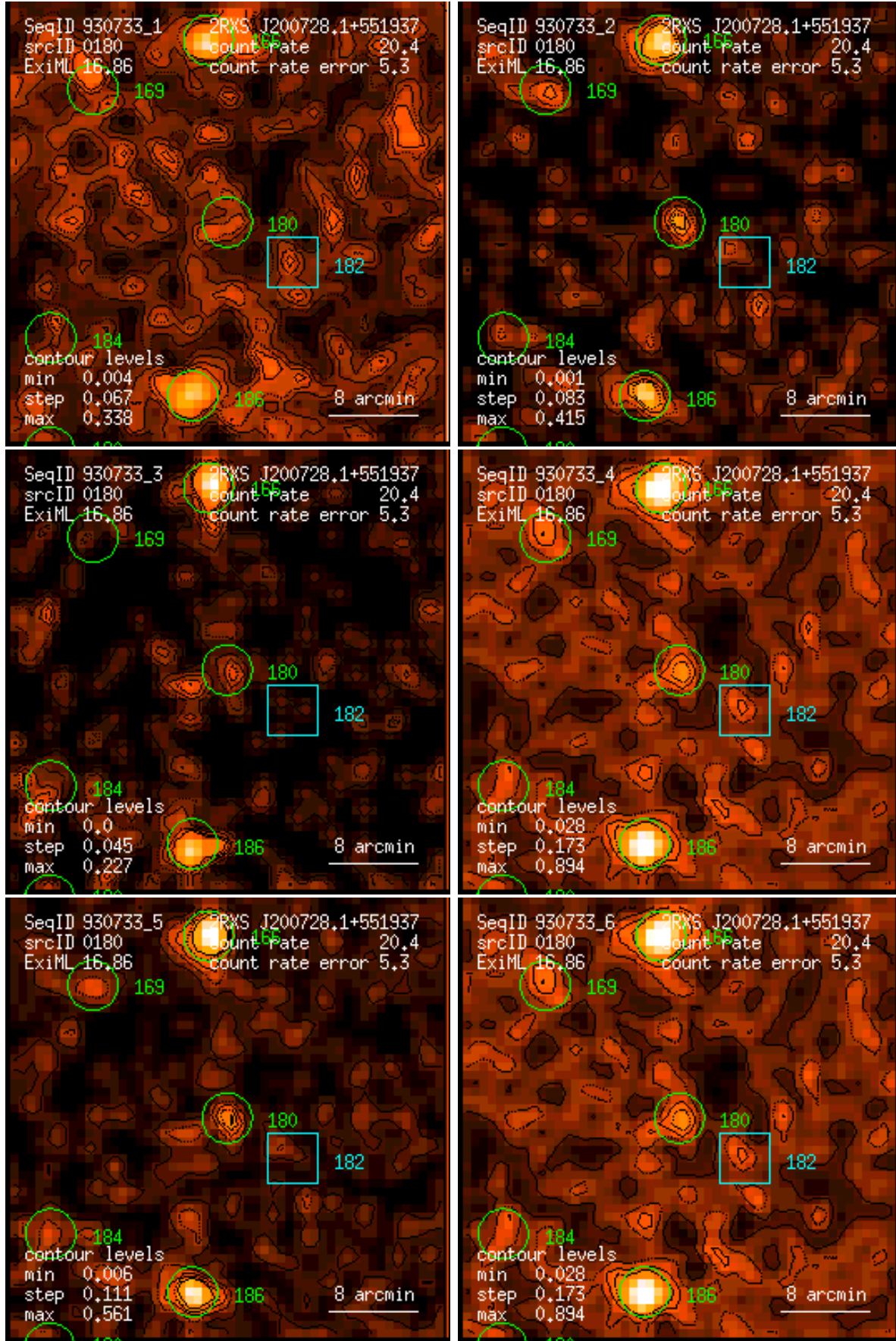
Figure 180: RASS 930733: detection 0180: band rate images, Gaussian filter: (1) PSPC channels 11 – 41, (2) 52 – 90, (3) 91 – 201, (4) 11 – 235, (5) 52 – 201, (6) 11 – 201. Broad band rates in counts/ks. Band rate contour levels in counts/ks/arcmin 2 .
