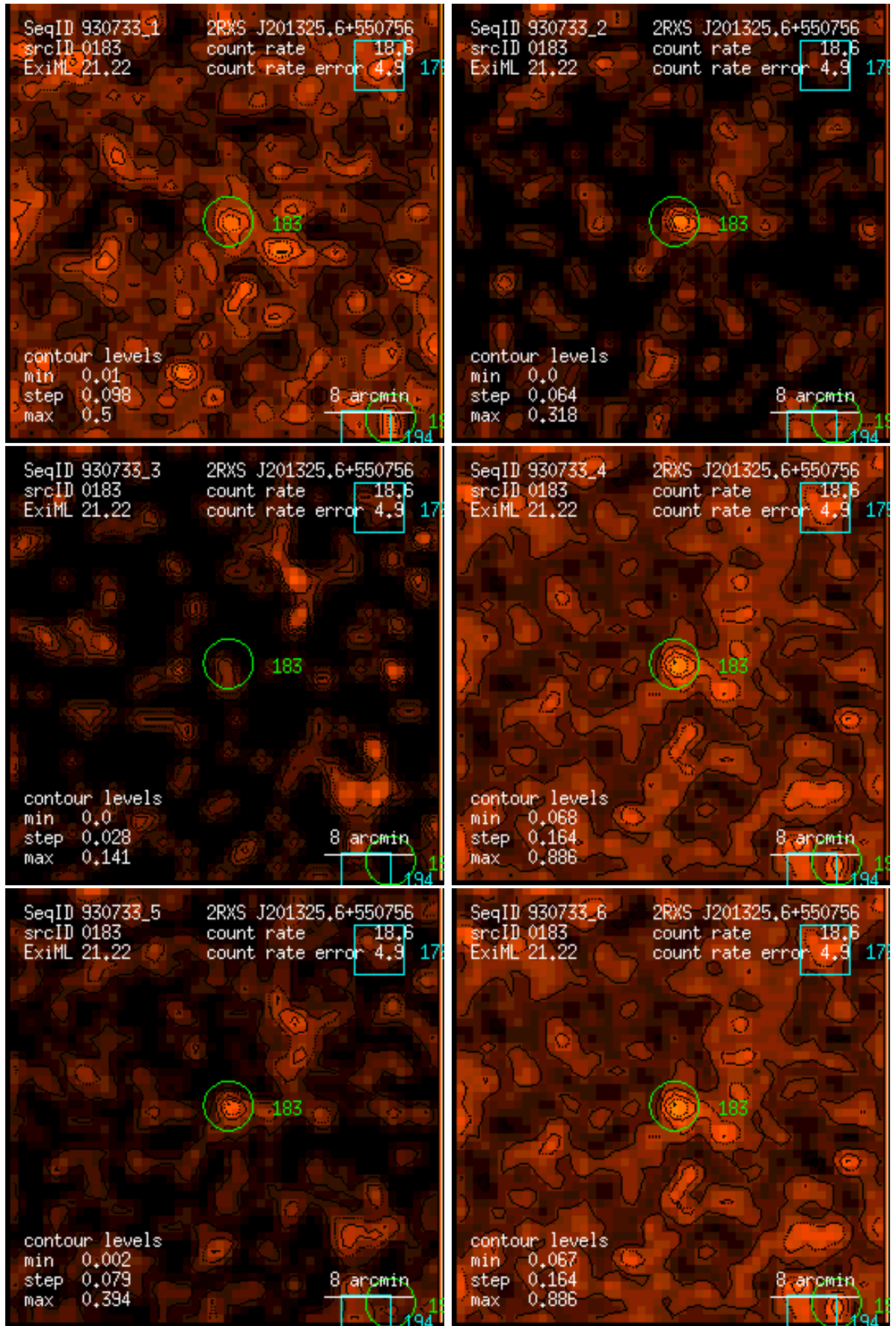
Figure 183: RASS 930733: detection 0183: band rate images, Gaussian filter: (1) PSPC channels 11 – 41, (2) 52 – 90, (3) 91 – 201, (4) 11 – 235, (5) 52 – 201, (6) 11 – 201. Broad band rates in counts/ks. Band rate contour levels in counts/ks/arcmin 2 .
