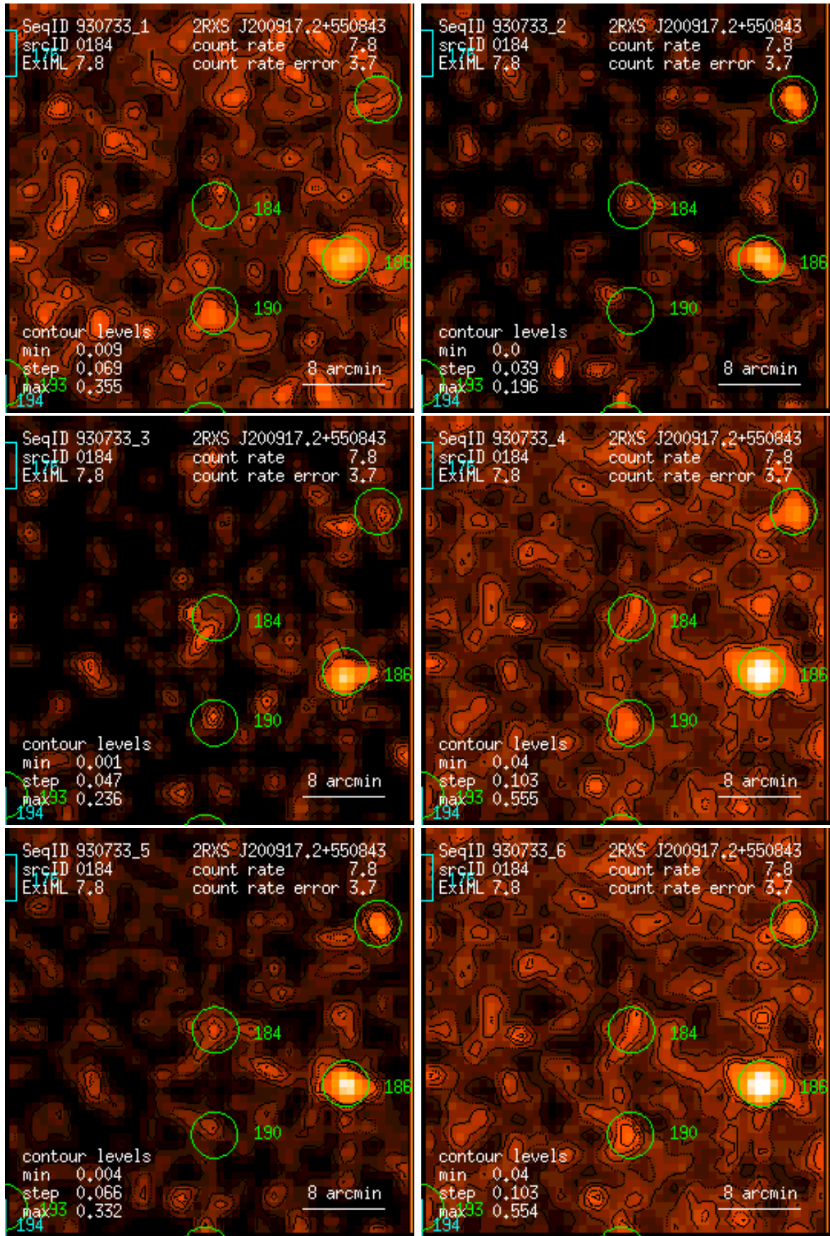
Figure 184: RASS 930733: detection 0184: band rate images, Gaussian filter: (1) PSPC channels 11 – 41, (2) 52 – 90, (3) 91 – 201, (4) 11 – 235, (5) 52 – 201, (6) 11 – 201. Broad band rates in counts/ks. Band rate contour levels in counts/ks/arcmin 2 .
