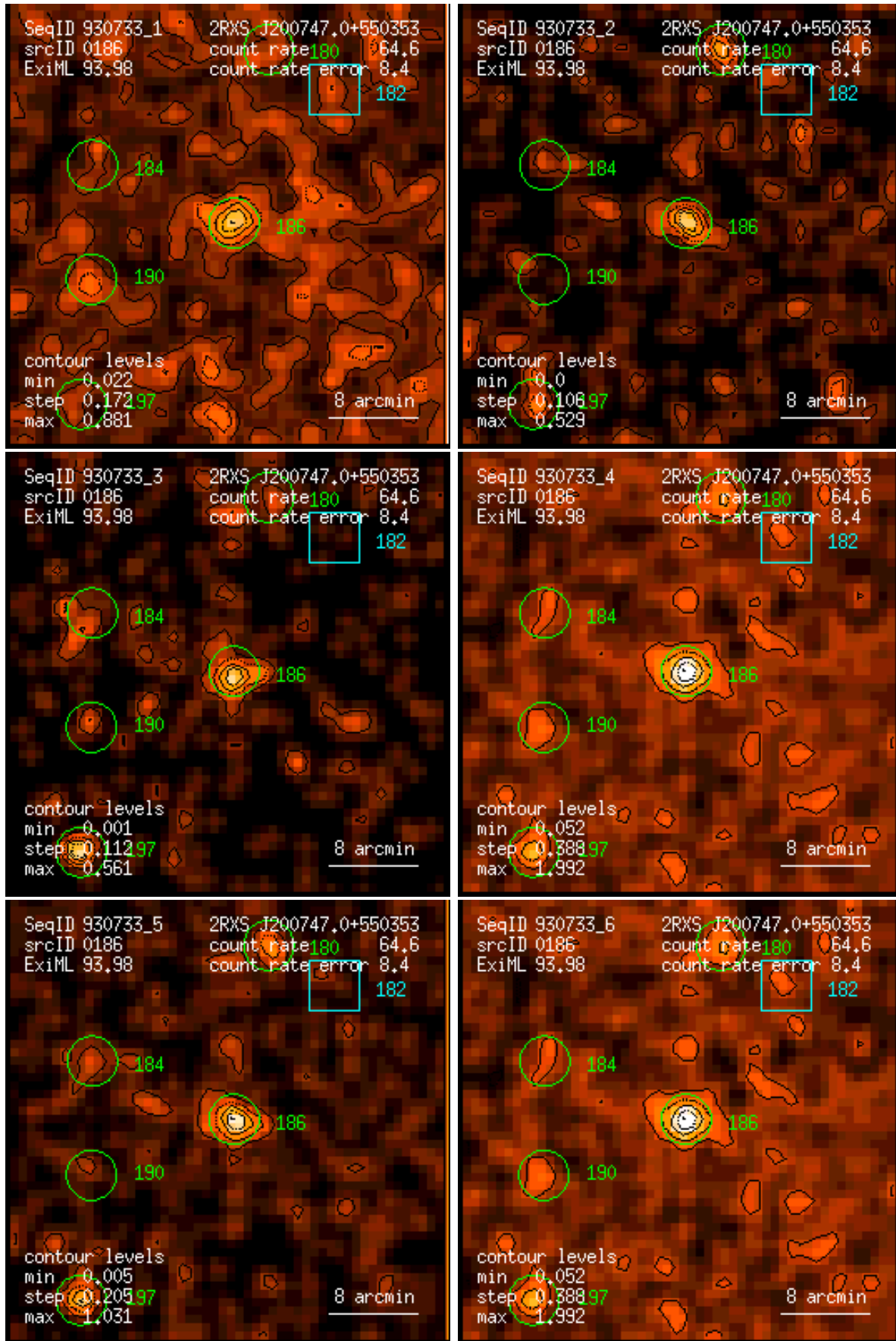
Figure 186: RASS 930733: detection 0186: band rate images, Gaussian filter: (1) PSPC channels 11 – 41, (2) 52 – 90, (3) 91 – 201, (4) 11 – 235, (5) 52 – 201, (6) 11 – 201. Broad band rates in counts/ks. Band rate contour levels in counts/ks/arcmin 2 .
