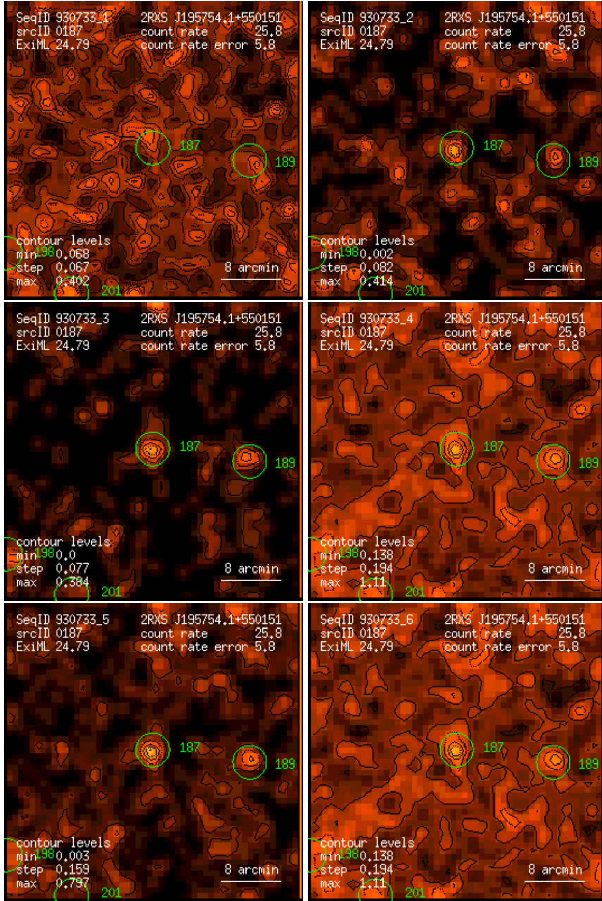
Figure 187: RASS 930733: detection 0187: band rate images, Gaussian filter: (1) PSPC channels 11 – 41, (2) 52 – 90, (3) 91 – 201, (4) 11 – 235, (5) 52 – 201, (6) 11 – 201. Broad band rates in counts/ks. Band rate contour levels in counts/ks/arcmin 2 .
