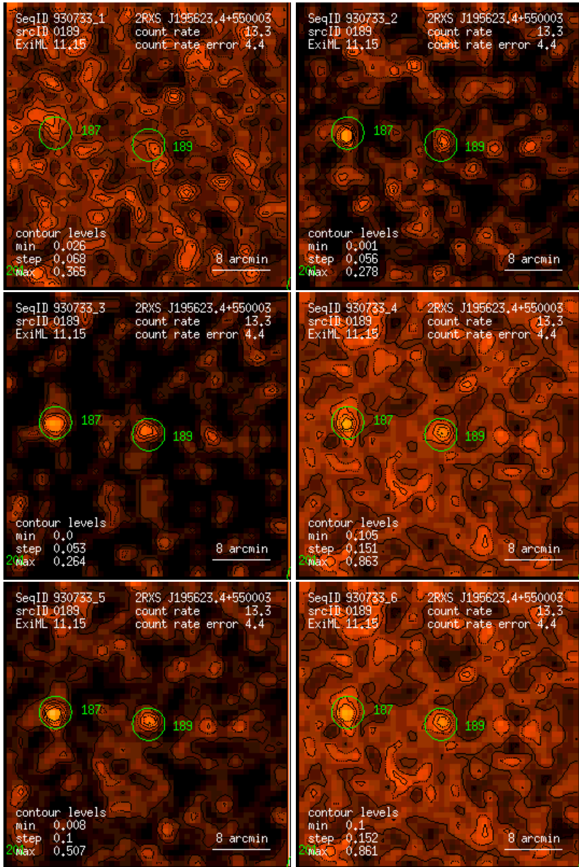
Figure 189: RASS 930733: detection 0189: band rate images, Gaussian filter: (1) PSPC channels 11 – 41, (2) 52 – 90, (3) 91 – 201, (4) 11 – 235, (5) 52 – 201, (6) 11 – 201. Broad band rates in counts/ks. Band rate contour levels in counts/ks/arcmin 2 .
