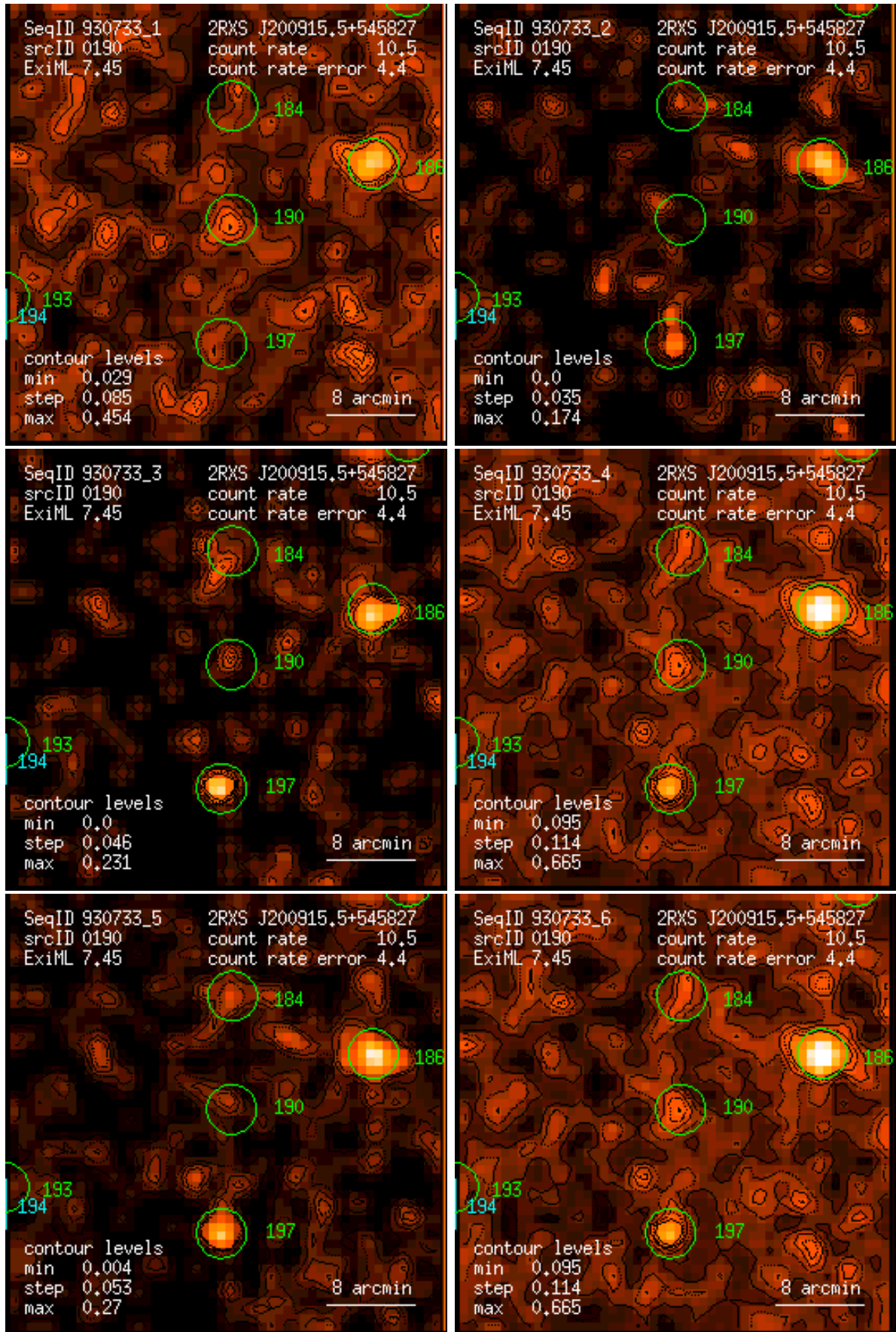
Figure 190: RASS 930733: detection 0190: band rate images, Gaussian filter: (1) PSPC channels 11 – 41, (2) 52 – 90, (3) 91 – 201, (4) 11 – 235, (5) 52 – 201, (6) 11 – 201. Broad band rates in counts/ks. Band rate contour levels in counts/ks/arcmin 2 .
