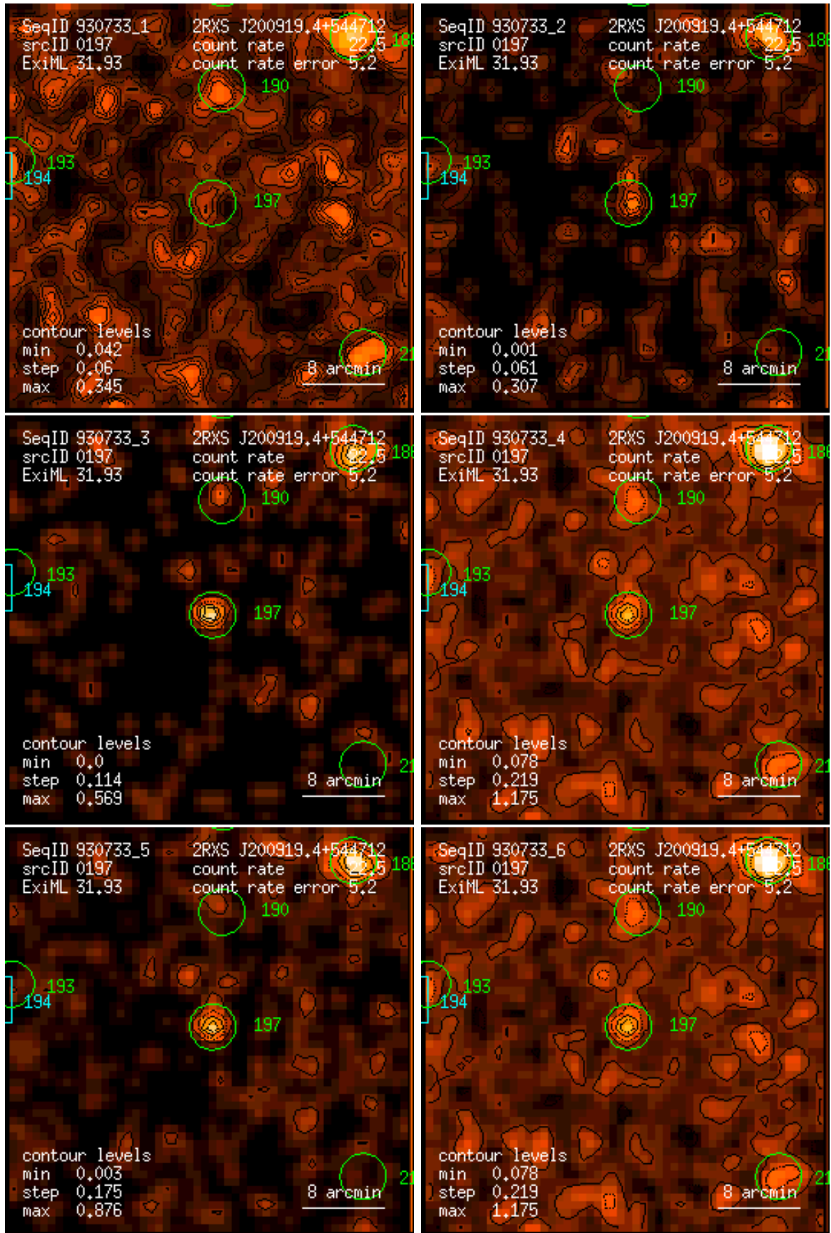
Figure 197: RASS 930733: detection 0197: band rate images, Gaussian filter: (1) PSPC channels 11 – 41, (2) 52 – 90, (3) 91 – 201, (4) 11 – 235, (5) 52 – 201, (6) 11 – 201. Broad band rates in counts/ks. Band rate contour levels in counts/ks/arcmin 2 .
