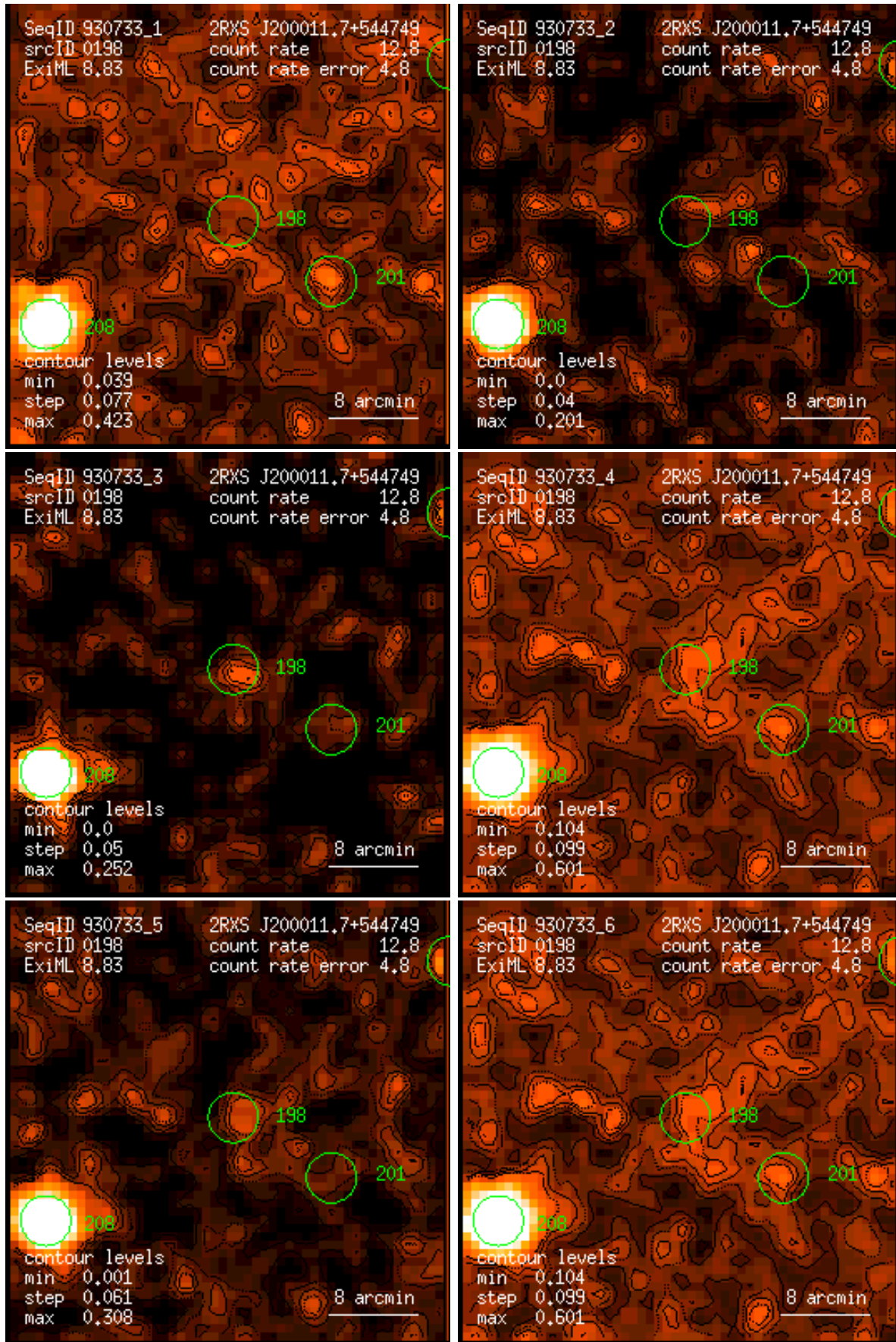
Figure 198: RASS 930733: detection 0198: band rate images, Gaussian filter: (1) PSPC channels 11 – 41, (2) 52 – 90, (3) 91 – 201, (4) 11 – 235, (5) 52 – 201, (6) 11 – 201. Broad band rates in counts/ks. Band rate contour levels in counts/ks/arcmin 2 .
