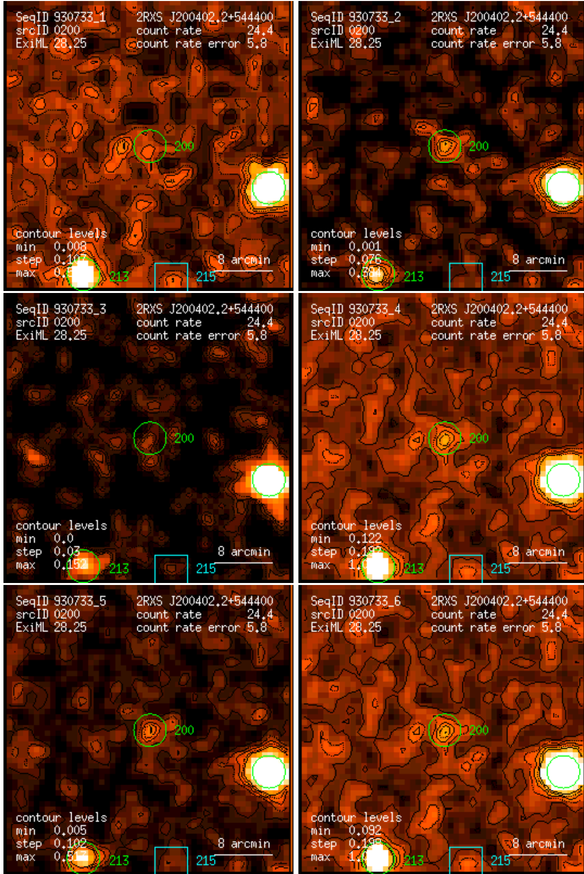
Figure 200: RASS 930733: detection 0200: band rate images, Gaussian filter: (1) PSPC channels 11 – 41, (2) 52 – 90, (3) 91 – 201, (4) 11 – 235, (5) 52 – 201, (6) 11 – 201. Broad band rates in counts/ks. Band rate contour levels in counts/ks/arcmin 2 .
