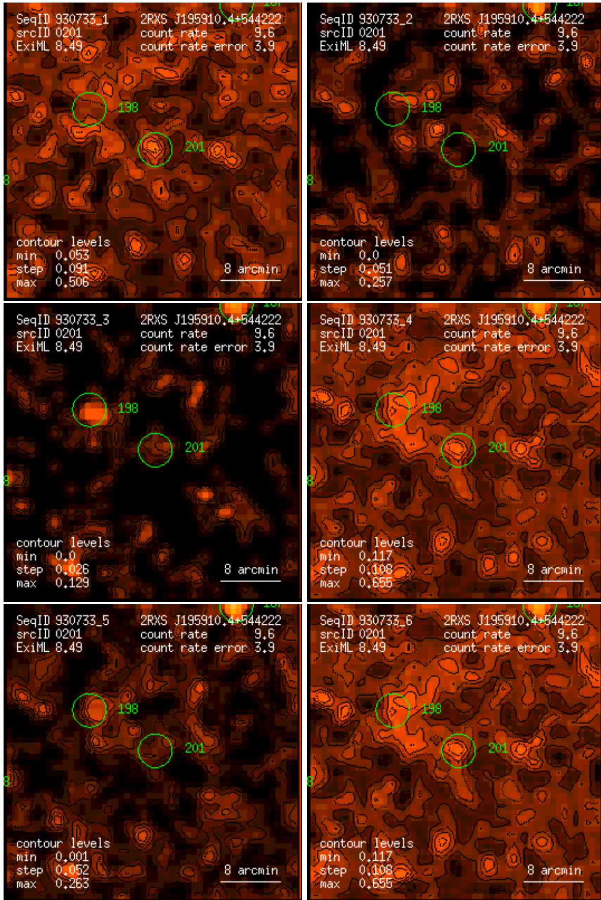
Figure 201: RASS 930733: detection 0201: band rate images, Gaussian filter: (1) PSPC channels 11 – 41, (2) 52 – 90, (3) 91 – 201, (4) 11 – 235, (5) 52 – 201, (6) 11 – 201. Broad band rates in counts/ks. Band rate contour levels in counts/ks/arcmin 2 .
