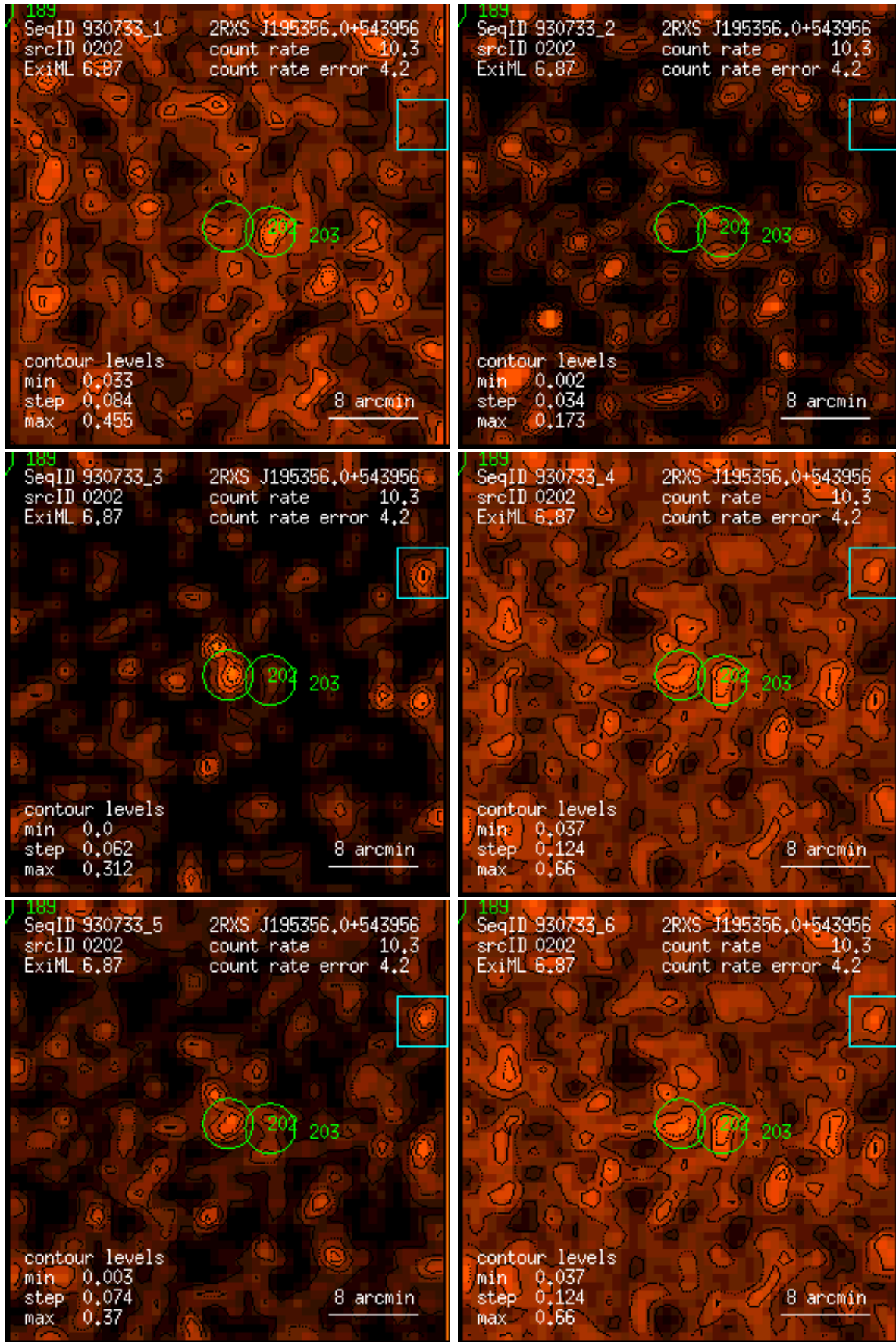
Figure 202: RASS 930733: detection 0202: band rate images, Gaussian filter: (1) PSPC channels 11 – 41, (2) 52 – 90, (3) 91 – 201, (4) 11 – 235, (5) 52 – 201, (6) 11 – 201. Broad band rates in counts/ks. Band rate contour levels in counts/ks/arcmin 2 .
