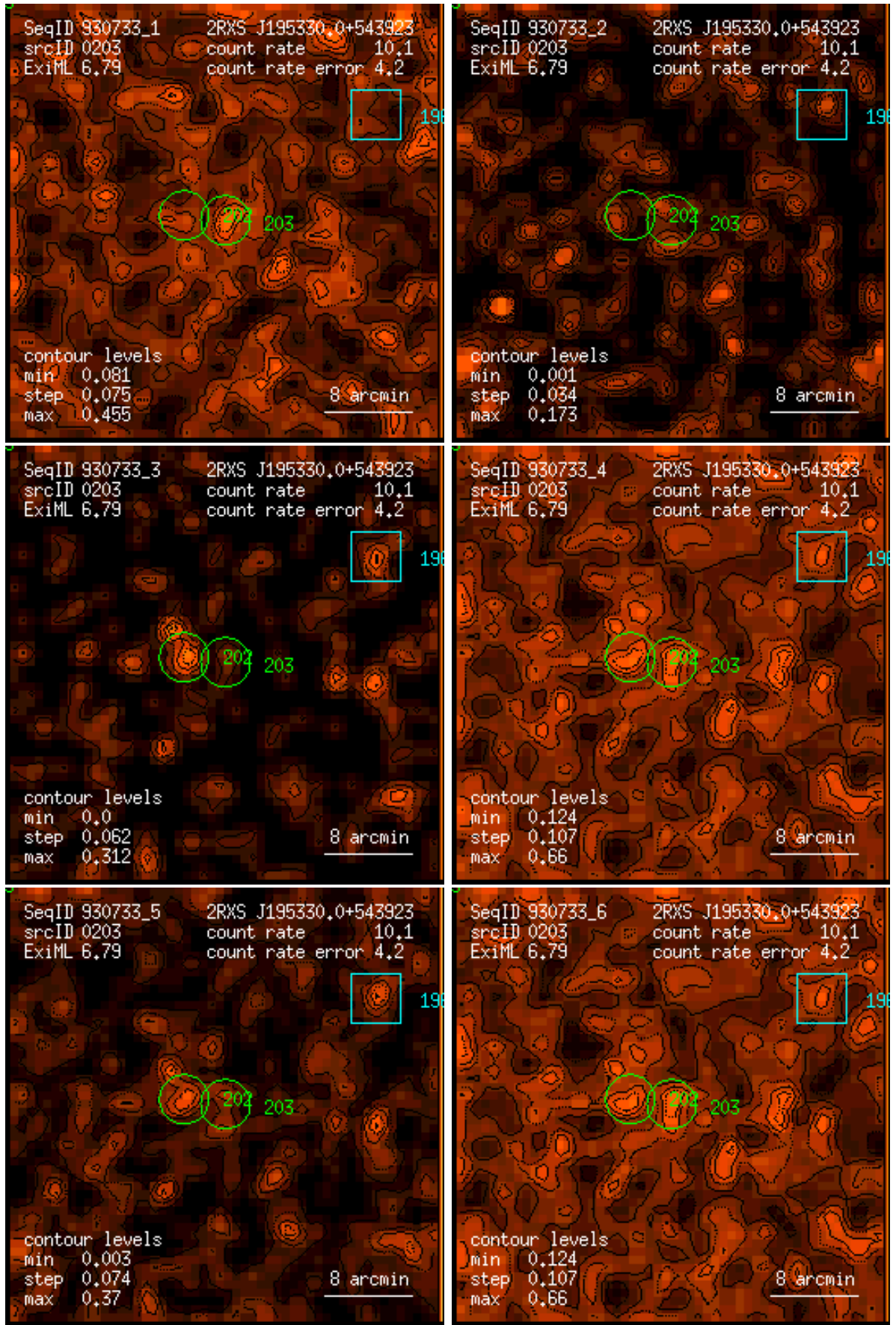
Figure 203: RASS 930733: detection 0203: band rate images, Gaussian filter: (1) PSPC channels 11 – 41, (2) 52 – 90, (3) 91 – 201, (4) 11 – 235, (5) 52 – 201, (6) 11 – 201. Broad band rates in counts/ks. Band rate contour levels in counts/ks/arcmin 2 .
