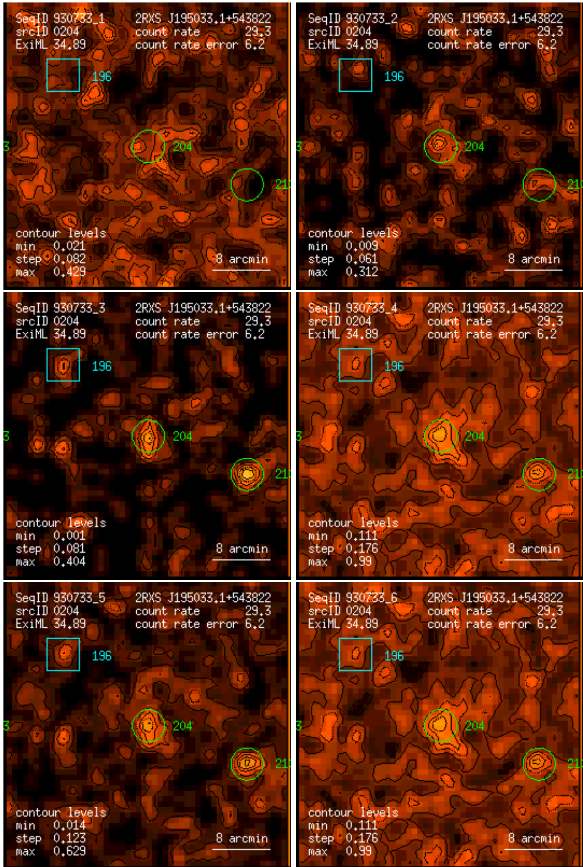
Figure 204: RASS 930733: detection 0204: band rate images, Gaussian filter: (1) PSPC channels 11 – 41, (2) 52 – 90, (3) 91 – 201, (4) 11 – 235, (5) 52 – 201, (6) 11 – 201. Broad band rates in counts/ks. Band rate contour levels in counts/ks/arcmin 2 .
